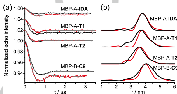
Figure 6. DEER results obtained with different tags on MBP mutants with (red) and without (black) one equivalent of maltose. (a) Background corrected DEER traces along with the fit obtained with the distance distributions shown on the right (grey). The uncorrected traces are shown in Figure S10 and corresponding RIDME results in Figure S11. (b) Analysed distance distributions.
