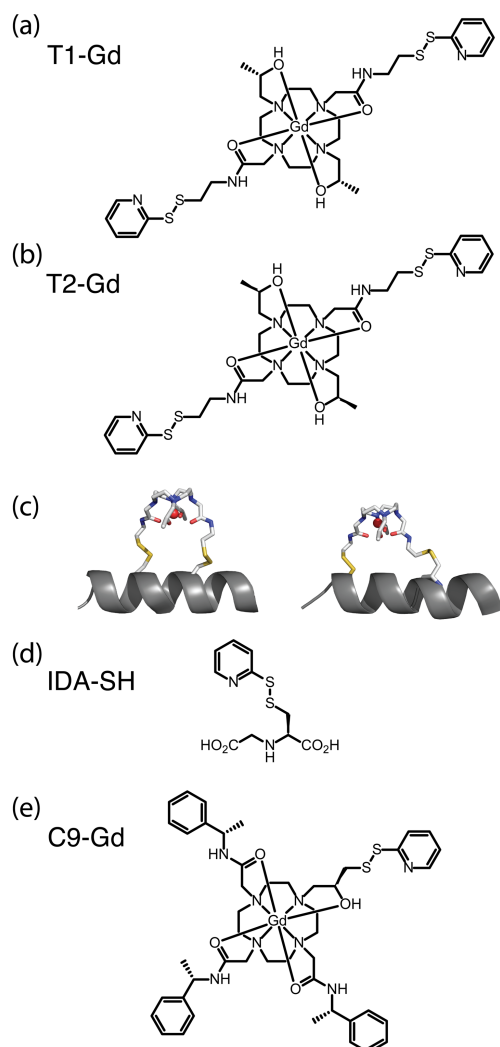
Figure 1. Structures of (a) T1-Gd tag (2-hydroxypropyl arms have S stereochemistry), (b) T2-Gd tag (2-hydroxypropyl arms have R stereochemistry), (c) T2-Gd tag modeled onto two cysteine residues in positions i and i +4 (left) or positions i and i +8 (right) of an \alpha -helix, (d) the IDA-SH tag activated by a thiopyridyl group for spontaneous reaction with a cysteine thiol group, and (e) the C9-Gd tag.
