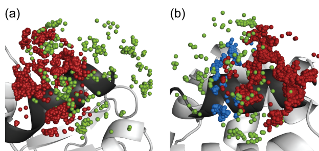
Figure 9. Comparison of \text{Gd}^{3+} ion coordinates predicted by modeling of T2-Gd and C9-Gd tags. Predicted metal positions are indicated by spheres. The helix carrying the tags is shown in dark grey. (a) Metal positions predicted for the site C341/C345 in MBP-A tagged with T2-Gd (red) and site C345 in MBP-B tagged with C9-Gd (green), using the crystal structure 1OMP. [28] (b) Metal positions predicted for the site C127/C131 in T4L-A tagged with T2-Gd (red), site C127/C135 in T4L-C tagged with T2-Gd (blue), and site C131 in T4L-D tagged with C9-Gd (green), using the crystal structure 2LZM. [26]
