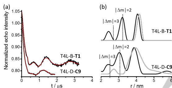
Figure 4. RIDME results obtained with T4L-B-T1-Gd and T4L-D-C9-Gd. (a) Background corrected RIDME traces (black) along with the fit obtained with the distance distributions shown on the right (red). The uncorrected traces are shown in Figure S4. (b) Comparison of the distance distributions obtained from the analysis of RIDME (black) and DEER (grey) data. The dotted lines show the positions expected for the second and third harmonics calculated from the main peak.
