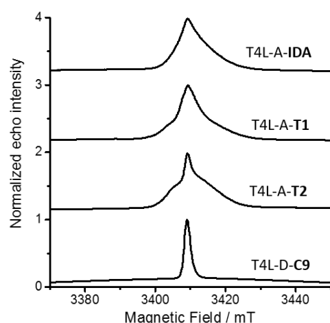
Figure 2. ED-EPR spectra of the central transition region, obtained for the \text{Gd}^{3+} ions in different tags attached to the T4 lysozyme mutants T4L-A and T4L-D. The ED-EPR spectra of the tags attached to the other mutants of T4L and MBP were similar and characteristic of the tag rather than the protein. All spectra were normalized to unity and are shifted by 1 for improved visualization and comparison.
