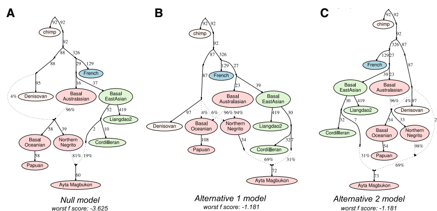
Figure 6. Admixture graph models of Denisovan introgression into Philippine Negritos and Papuans
