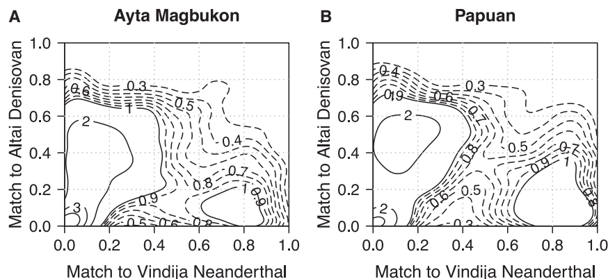
Figure 5. Contour density plots showing the affiliation of S'-detected introgressed segments to the reference archaic genomes
