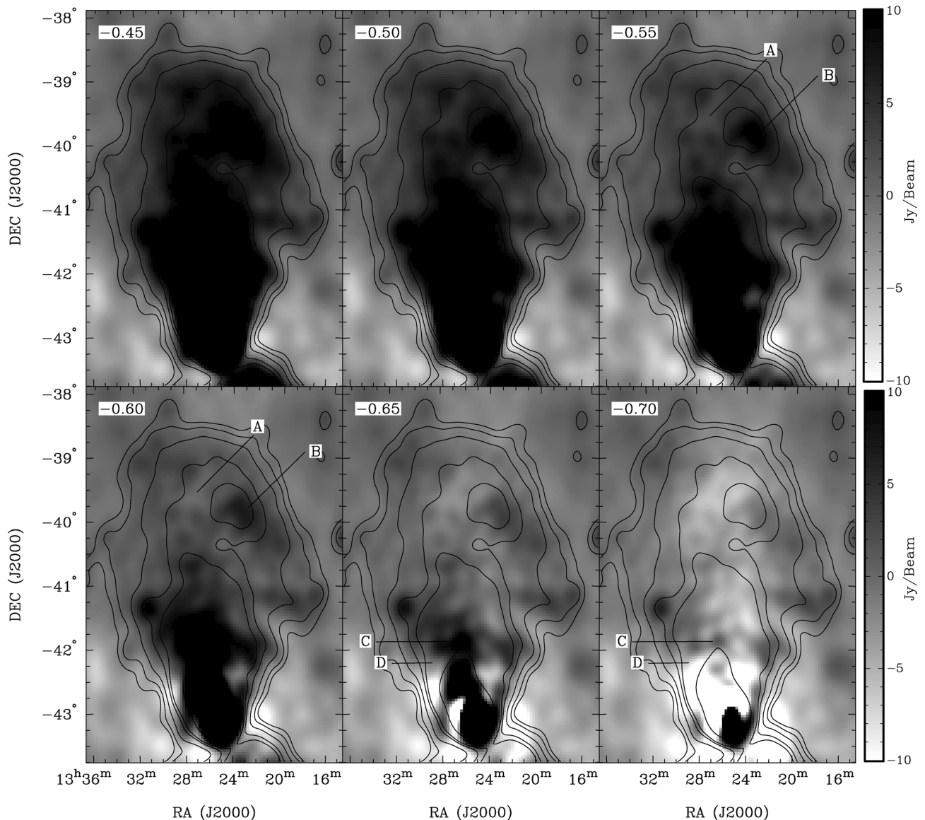
Figure 9. A subset of the spectral tomography images of the northern lobe between 118 MHz and 1.4 GHz with trial spectral indices as indicated in the top-left corner of each sub-image. Grey-scale is from -10 to 10 \text{ Jy beam}^{-1} . Overlaid are contours from the 118 MHz image at 2.5, 5, 10, 20, 28.3 and 113 \text{ Jy beam}^{-1} . The feature labelled A has a significantly flatter spectral index than that labelled B. Similarly, there is a change in spectral index between the flatter region labelled D and the steeper feature labelled C.
