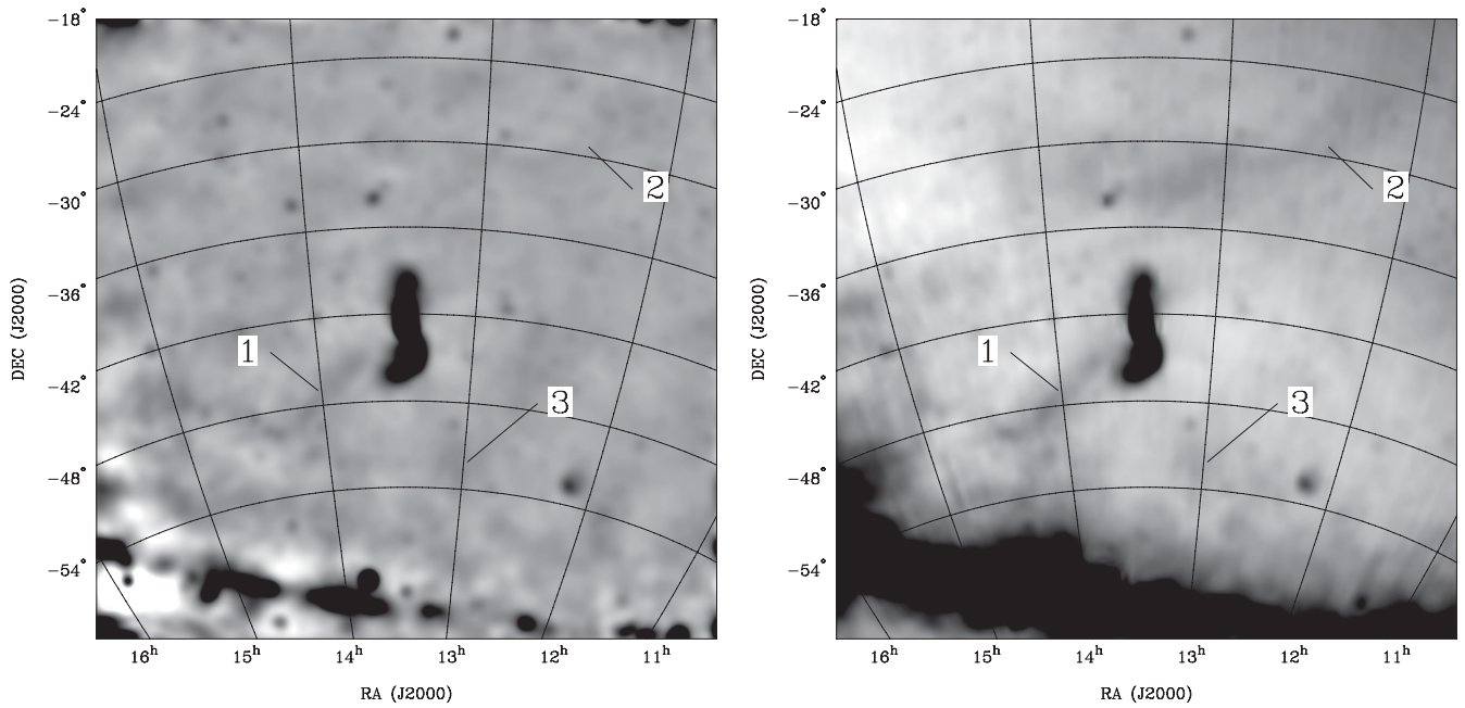
Figure 5. Comparison between the MWA 118 MHz image (left) and Haslam et al. (1982) 408 MHz image (right), both smoothed to the same angular resolution of 0''.85 . A linear brightness gradient has been subtracted from the Haslam et al. (1982) map to make the smaller-scale structures clearer. The faint diffuse structure on scales less than 12'' matches well by eye. Labels 1 to 3 indicate large-scale foreground features clearly present in both maps.
