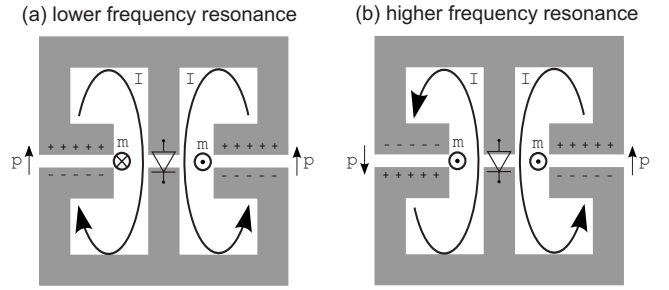
FIG. 4. Resonant modes of the electric resonators, showing the two current loops I and their electric and magnetic dipole moments p and m , respectively.
