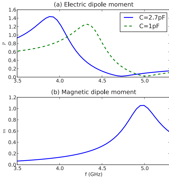
FIG. 5. (Color online) Numerically calculated (a) electric and (b) magnetic dipole moments of the resonator aligned parallel to \vec{k} .
