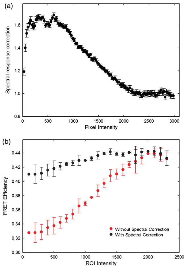
Fig. 9 Instrument spectral response correction: (a) The spectral response correction [G(I)] related to the normalized ratio of donor to acceptor emission intensities in a sample with fixed FRET efficiency is plotted against the maximal acceptor emission intensity of each pixel. (b) The average FRET efficiency for cells expressing C5V is shown using only ROIs that have average acceptor intensity above the value shown on the x-axis, before (red) and after (black) instrument spectral response correction.
