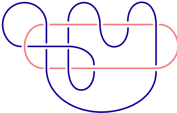
Figure 1.4. The link used in Theorem 4.4 is L12n1314 in the Hoste-Thistlewaite census. Our framing conventions for Dehn filling are \curvearrowright and are consistent with SnapPy [CDW]. Note there is an orientation-preserving homeomorphism of S^3 which interchanges the two components.
