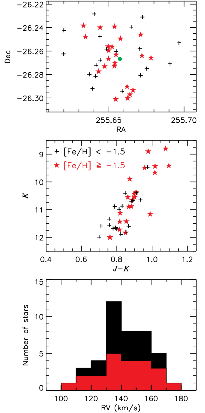
Figure 8. Spatial distribution (upper), CMD (middle) and RV distribution (lower). Black crosses and red stars represent objects with [\text{Fe}/\text{H}] < -1.5 and [\text{Fe}/\text{H}] \geq -1.5 , respectively.
