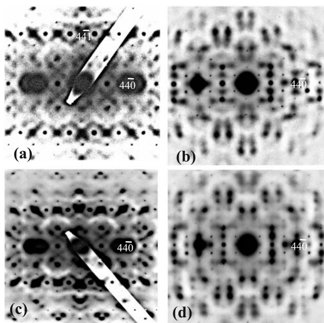
Fig. 1 Typical \langle 118 \rangle zone axis EDPs obtained from (a) BZN and (c) BZSN ( x=1.0 ), by tilting \sim 10^\circ away from the \langle 001 \rangle zone axis keeping the \langle -2, -2, 0 \rangle^* systematic row excited and \sim \langle 511 \rangle zone axis EDPs obtained from (b) BZN and (d) BZTN ( y=1.5 ) by tilting \sim 8^\circ away from the exact \langle 110 \rangle zone axis orientation again keeping the \langle -2, -2, 0 \rangle^* systematic row excited
