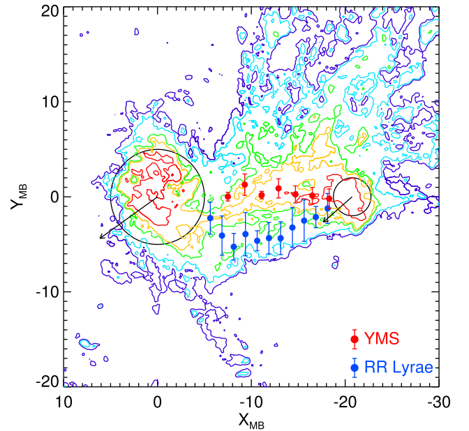
Figure 15. The three Magellanic bridges in the MB coordinate system. Contours give the density of the H I gas in the velocity range 100 < V_{\text{LOS}} (\text{km s}^{-1} < 300) . Red, yellow, green, blue and purple contours correspond to gas column density of (12.02, 3.18, 1.80, 0.46, 0.16) \times 10^{-20} \text{ cm}^{-2} . Blue (red) filled circles with error bars give the evolution of the centroid and the width of the RR Lyrae (YMS) bridge as a function of the MB coordinates. Blue filled circles with error bars show the evolution of the centroid and the width of the RR Lyrae bridge. The LMC and the SMC are shown as large circles. Arrows give the proper motion vectors of the Clouds from Kallivayalil et al. (2013) in the MB coordinate system.
