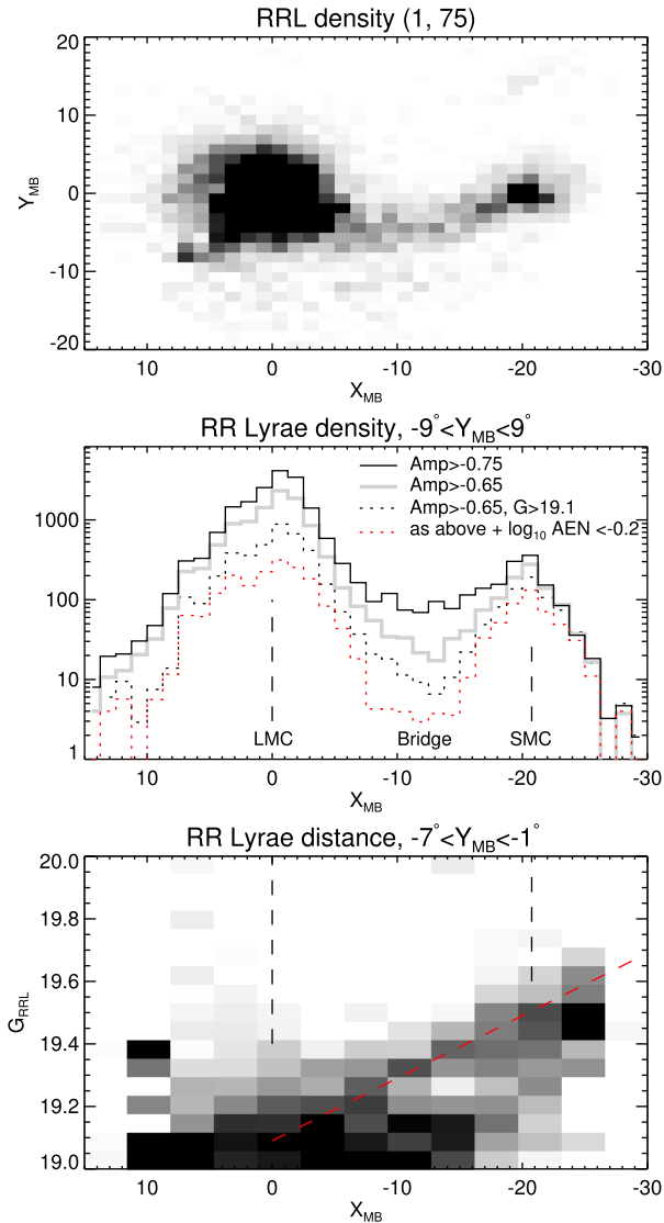
Figure 10. Top: density of the Gaia RR Lyrae candidates in the MB coordinate system in which both the LMC and the SMC lie on the equator. The pixel size is 1^{\circ}25 on a side. Middle: density of the RR Lyrae candidate stars along the MB equator. A foreground/background model (linear along MB latitude Y_{MB} and different for each X_{MB} ) is subtracted. The inset explains the cuts applied for each of the histograms. Bottom: variation of the apparent magnitude of the RR Lyrae along the bridge. For these RR Lyrae, a stricter cut on variability amplitude was applied, namely \text{Amp} > -0.65 . Between the LMC and the SMC, two structures at distinct distances are visible: one at the distance of the LMC, i.e. at G \sim 19 and one connecting the LMC and the SMC (at G \sim 19.5 ). Red dashed line gives the approximate behaviour G = 19.02 - 0.2X_{MB} of the more distant of the two RR Lyrae structures.
