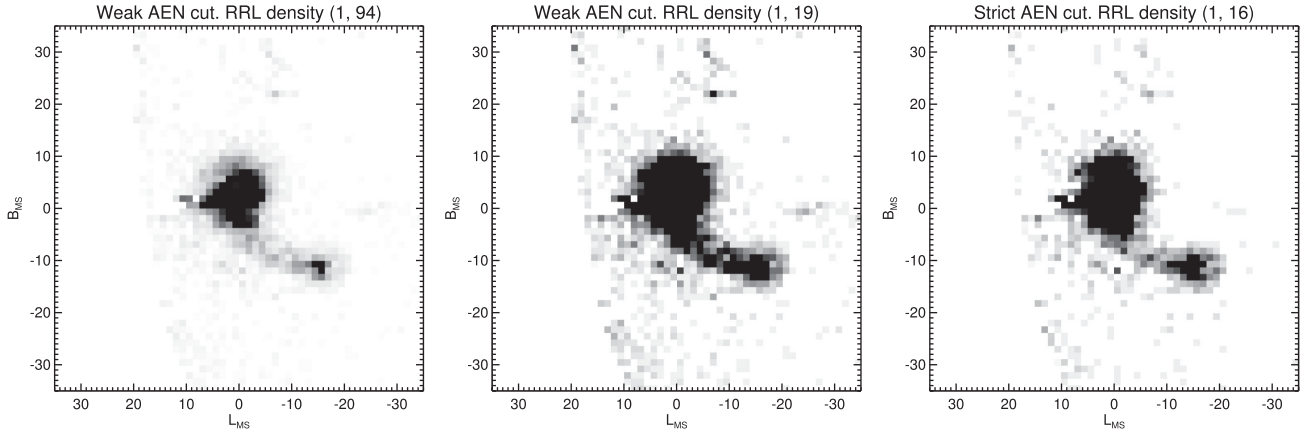
Figure 8. Density of the RR Lyrae candidate stars in 70^\circ \times 70^\circ area centred on the LMC in the MS coordinate system. Pixels are 1.25'' on a side. The pixel values corresponding to black and white are given in brackets in the title of each panel. Left and centre: \sim 23\,000 stars selected using (amongst others) a \log_{10}(\text{AEN}) < 0.25 cut (see Fig. 4 for details). The difference between the two panels is only in the maps’ dynamic range as indicated in the panel titles. Both Clouds are clearly visible as well as a bridge connecting them, with a cross-section roughly matching that of the SMC. Right: density map of the 10501 RR Lyrae candidates selected using a stricter \log_{10}(\text{AEN}) < -0.2 cut. Here, most of the artefacts related to the cross-match visible in the centre panel disappear, albeit at the expense of the noticeable reduction in the sample size.
