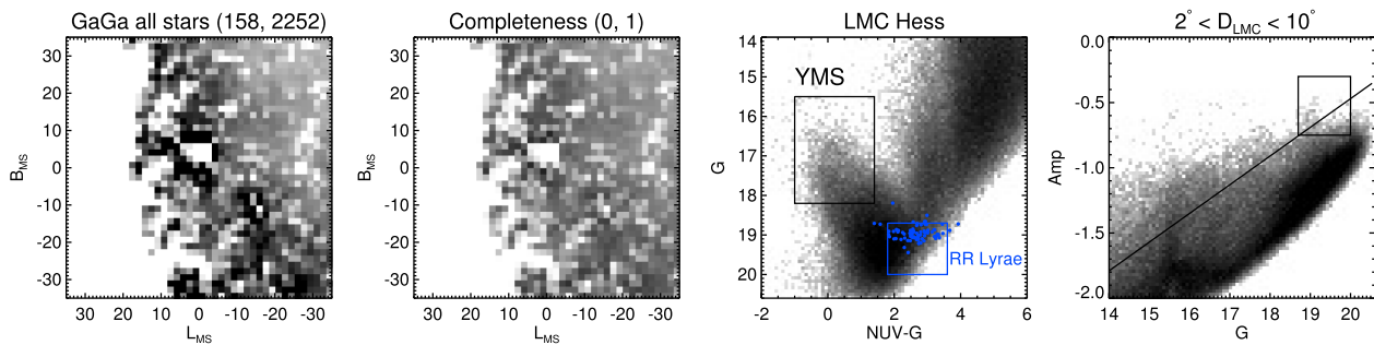
Figure 11. Selecting Magellanic RR Lyrae and YMS stars with GaGa = Gaia + GALEX . First panel: density map of stars with both Gaia and GALEX detections. The pixel size is 1''.667 on a side. Second panel: completeness map of GaGa. Third panel: logarithm of density in the colour–magnitude space (Hess diagram) spanned by G and NUV - G for stars with 2^\circ < D_{\text{LMC}} < 10^\circ . Two selection boxes are shown: one aimed at identifying Magellanic RR Lyrae stars (blue) and one for YMS stars (black). Fourth panel: logarithm of density of GaGa sources in the space spanned by Amp and G for a region around the LMC. The LMC RR Lyrae are clearly identified in the designated selection box. Note that we use a slightly different cut on astrometric excess noise, i.e. \log_{10}(\text{AEN}) < -0.1 .
