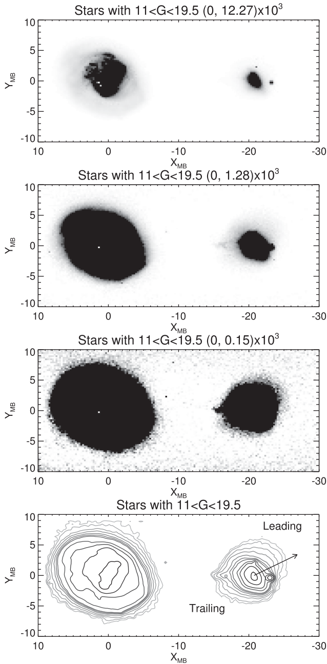
Figure 2. Density of stars with 11 < G < 19.5 in the MB coordinate system. The pixels are 0.25^\circ \times 0.25^\circ . A background model comprising a quadratic polynomial for each column (constrained over the range of -13^\circ < X_{\text{MB}} < 35^\circ , but excluding -8^\circ < X_{\text{MB}} < 8^\circ ) is subtracted. Across all panels, the density distribution is the same, only the dynamic range of the pixel values changes. The number of stars corresponding to white (low counts) and black (high counts) levels is shown in brackets in the title of each panel. First (top) panel: note the perturbed disc of the LMC. Second panel: note the low surface-brightness extension of the SMC, the 47 Tuc cluster in the western part of the dwarf and the Wing in the eastern side, facing the LMC. Third panel: note the characteristic S-shape of the outer envelope of the density distribution of the SMC. Fourth (bottom) panel: note the twist of the iso-density contours from the centre outwards. The two protruding ends of the S-shape are the origins of the SMC tidal tails. The arrow shows the Cloud’s proper motion relative to the LMC as computed using the values from Kallivayalil et al. (2013). The solar reflex motion is subtracted. The leading and trailing tails are marked taking into account the direction of the SMC’s motion around the LMC.
