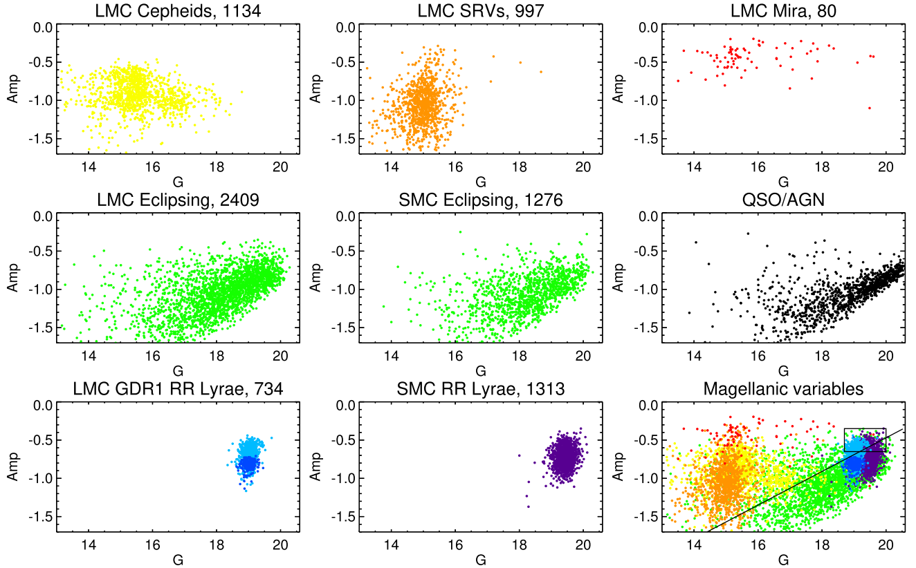
Figure 3. Variable sources in Gaia DR1. Previously identified objects with secure classification are shown in the plane spanned by the variability amplitude Amp and the Gaia magnitude G . The title also reports the number of variables shown. Top left: LMC Cepheids with 3^\circ < D_{\text{LMC}} < 10^\circ from Soszynski et al. (2008). Top centre and right: long-period SRVs and Mira stars in the LMC from Soszyński et al. (2009) with 3^\circ < D_{\text{LMC}} < 10^\circ . Middle left: LMC eclipsing binaries with 3^\circ < D_{\text{LMC}} < 10^\circ from Graczyk et al. (2011). Middle centre: SMC eclipsing binaries with D_{\text{SMC}} > 1^\circ from Pawlak et al. (2013). Middle right: QSO and AGN from Véron-Cetty & Véron (2010). Bottom left: Gaia DR1 RR Lyrae with 5^\circ < D_{\text{LMC}} < 10^\circ (see Clementini et al. 2016, for details). RRAb (RRc) stars are shown in light (dark) blue. Bottom centre: RR Lyrae in the SMC with D_{\text{SMC}} > 1^\circ from Soszyński et al. (2010). Bottom right: all Magellanic variables from other panels. Black lines show the RR Lyrae selection boundaries used in the analysis. This selection yields 38 per cent completeness for the LMC RR Lyrae and 13 per cent completeness for the SMC RR Lyrae. Note that the variables shown in this figure also had to pass the additional cuts detailed in Section 3.3.
