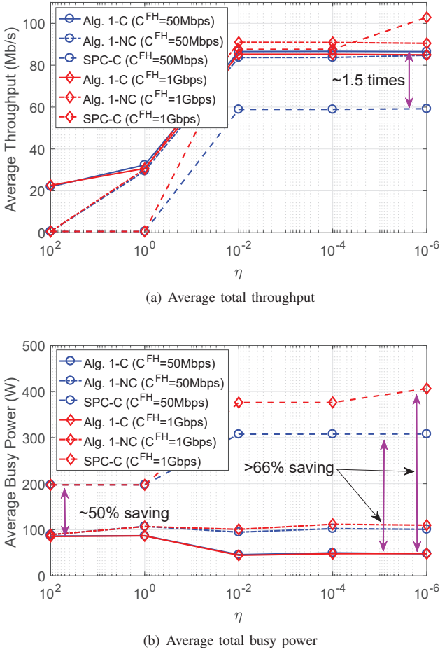
Fig. 3. Effects of joint design, local caching and limited backhaul capacity on network performance
