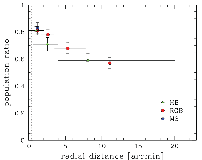
Figure 33. Radial distribution of the fraction of HBb (green triangles), RGBb (red circles), and MSb stars (blue square) with respect to the total number (component a + component b ) of HB, RGB, and MS stars, respectively. The horizontal lines indicate the radial extent of the region corresponding to each measure. Vertical dotted and dashed lines mark the core and the half-mass radius, respectively.
