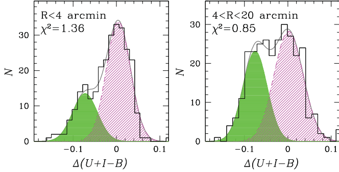
Figure 29. Histogram of the \Delta(U+I-B) distribution of HB stars from ground-based photometry at two radial distances from the cluster center.
