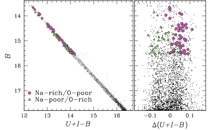
Figure 26. Na-poor/O-rich and Na-rich/O-poor RGB stars defined in Figure 24 are plotted here in B vs. U+I-B (left panel); the right-hand panel shows a verticalized version in our usual way.
