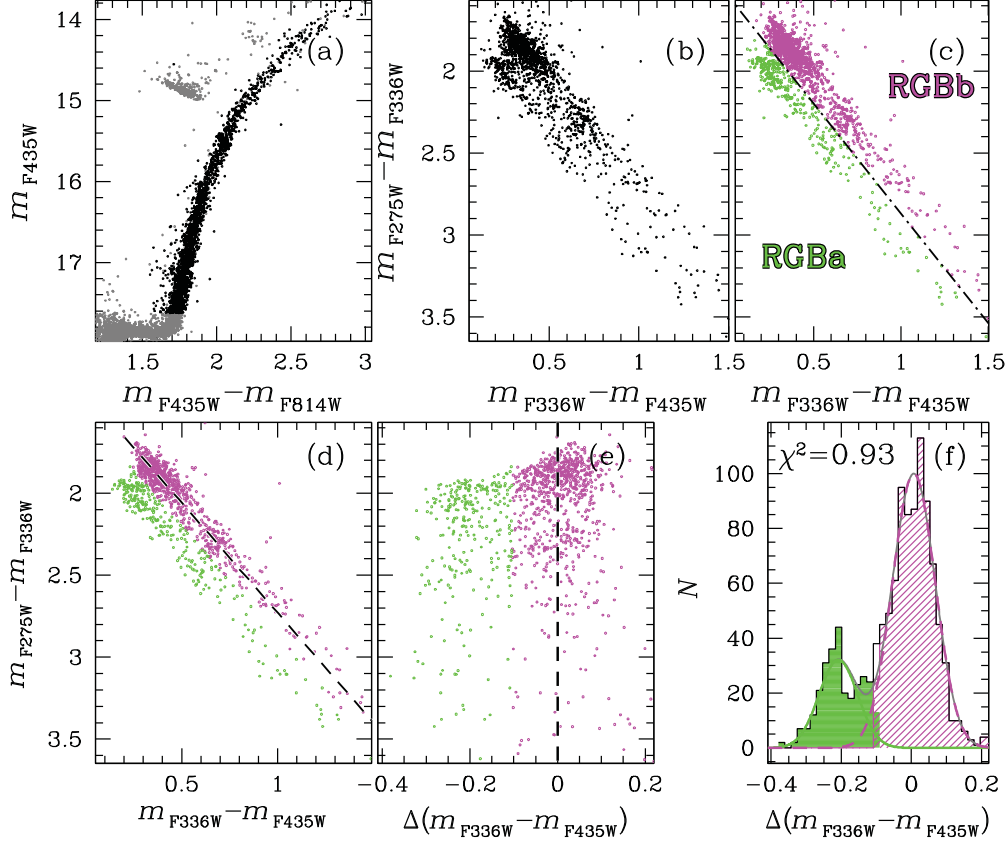
Figure 16. Panel (a): m_{F435W} vs. m_{F435W} - m_{F814W} CMD from ACS/WFC photometry. The black points are the RGB stars that we show in the other panels. (b) m_{F275W} - m_{F336W} vs. m_{F336W} - m_{F435W} two-color diagram for these stars. (c) We arbitrarily drew by hand the dash-dotted line that separates RGBa (green) and RGBb (magenta). (d) The dashed line is the fiducial sequence of the RGBb stars, drawn by the fitting method that we described in Section 3. (e) The verticalized colors of the stars. (f) Histogram of the colors in panel (e), with a fit by two Gaussians, whose sum is shown by the solid gray line.
