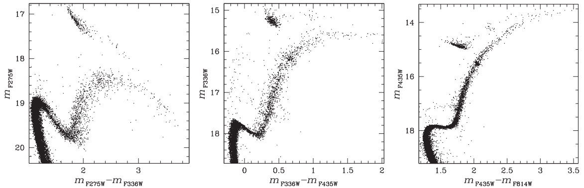
Figure 15. This figure illustrates the three CMDs from HST photometry that best summarize the behavior of RGB stars. Note the wide color spread of \sim 0.1 – 0.2 mag in the left and the middle CMDs, which also show some hints of color bimodality. The RGB becomes narrower and well defined in the right-hand CMD.
