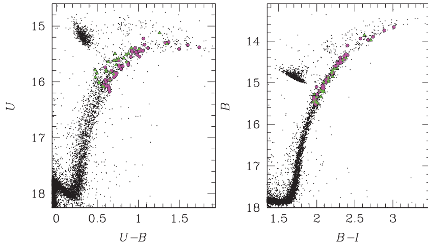
Figure 25. U vs. U-B (left panel) and B vs. B-I (right panel) CMD from ground-based photometry. The stars belonging to the two groups of Na-rich (O-poor) and Na-poor (O-rich) stars are represented with magenta circles and green triangles, respectively.
