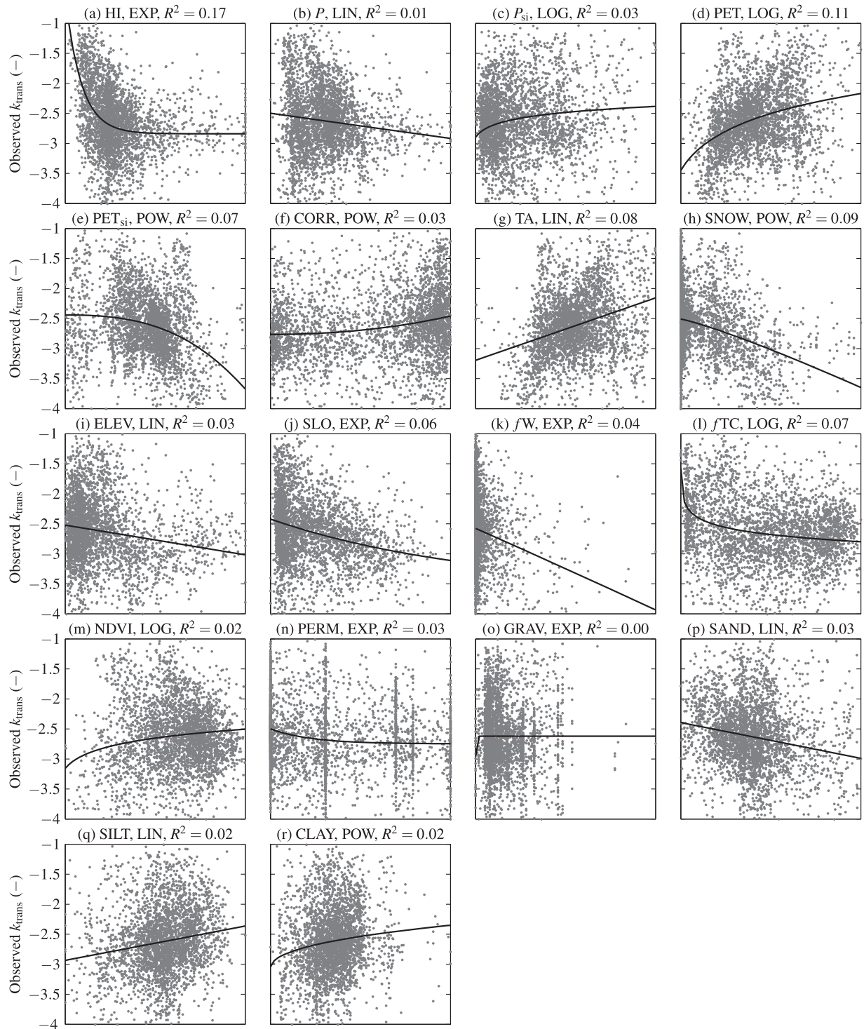
Figure 7. Scatterplots of catchment-mean values of the climatic and physiographic characteristics (along the x axis) versus the observed k_{\text{trans}} (along the y axis), including the best-fit regression line. Each data point represents a catchment ( n = 3394 ). The x axis is linear and ranges from the minimum to maximum value of the data (not shown). Table 1 lists descriptions of the predictor variables. Abbreviations referring to the type of regression equation: EXP, exponential; LIN, linear; LOG, logarithmic; and POW, power.
