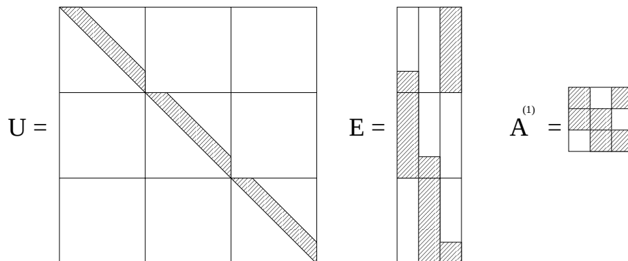
FIGURE 7.3. Matrices involved in a block elimination step
