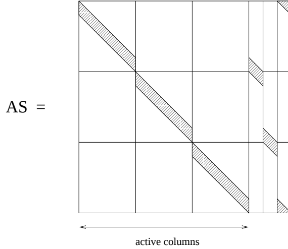
FIGURE 7.2. Permutation AS of matrix A from Figure 7.1
