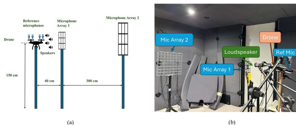
Fig. 2. Drone directional ANC system experiment setup (a) experiment layout (b) experiment photo.
