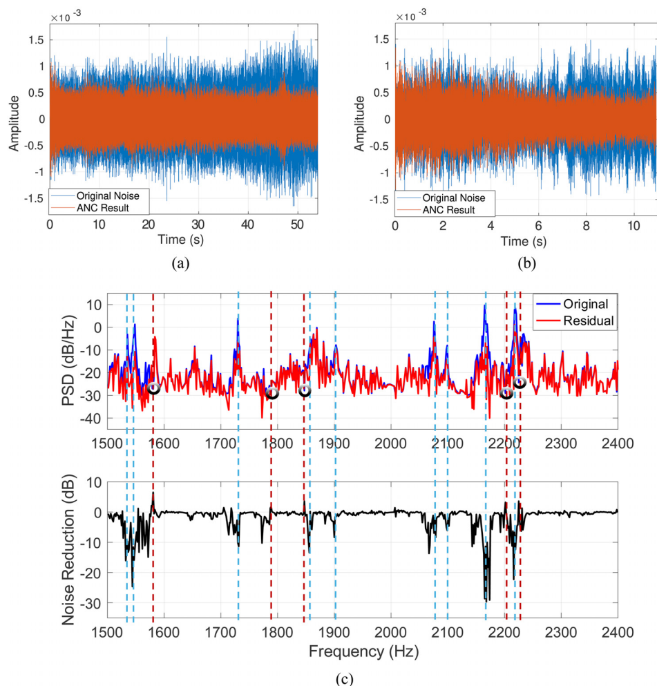
Fig. 4. Drone ANC results in the time and frequency domains. (a) Tuning data: ANC performance using the same noise recording as in the tuning stage. (b) Testing data: performance using a different segment of the noise recording. (c) PSD with an arbitrary reference and noise reduction at one of the virtual microphones with testing data, demonstrating approximately 10 dB attenuation within the target frequency band. The red dotted lines indicate positive noise reduction values, which occur where the original noise level was very low.
