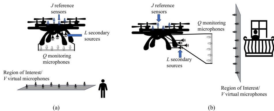
Fig. 1. Drone directional ANC system setup (a) reducing noise downward and (b) reducing noise sideways: Q monitoring microphones hanging on the drone, L secondary sources mounted on the drone fuselage, J reference sensors placed near the drone propellers, and V virtual microphones sample the ROI in the far-field.
