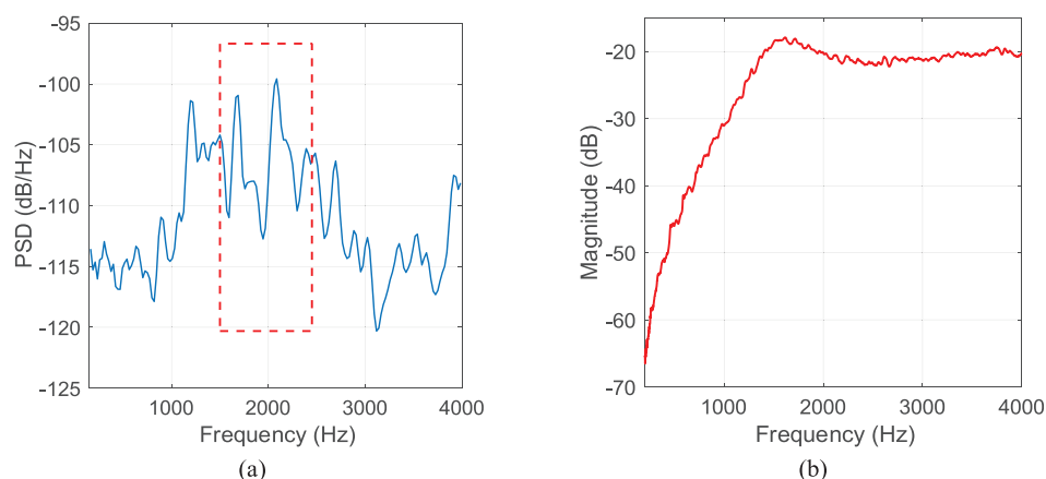
Fig. 3. Justification for sub-band processing: (a) PSD with an arbitrary reference observed at the virtual microphone, showing dominant blade-passage frequency components in the 1500–2400 Hz range. (b) Measured magnitude response (with an arbitrary reference) of the ND20FA-6 loudspeaker, exhibiting a flat response above 1500 Hz and a noticeable roll-off below.
