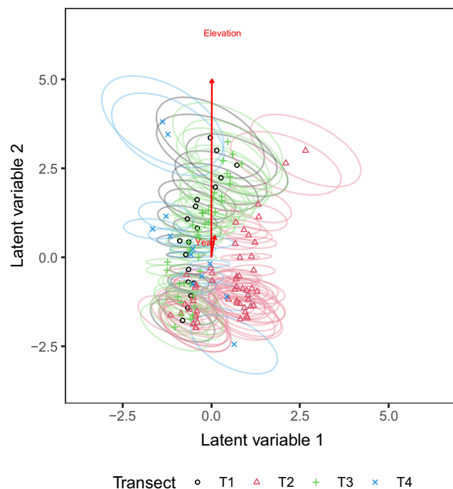
FIGURE 3 Concurrent ordination plot for sites from the Skabbholmen dataset, conditional on a random row intercept to account for pseudoreplication of transects. Sites with corresponding 95% prediction regions are coloured by their respective transects. Estimates and standard errors of the canonical coefficients are provided in Table S4 of Appendix S7.
