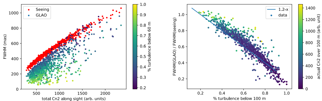
Figure 8. Left: Scatterplot showing seeing limited and GLAO corrected FWHM as a function of total turbulence. The colour of the GLAO points encode the fraction of turbulence below 60 m. Right: GLAO correction ratio (ratio of FWHM GLAO to seeing limited) as a function of the fraction of turbulence below 100 m.
