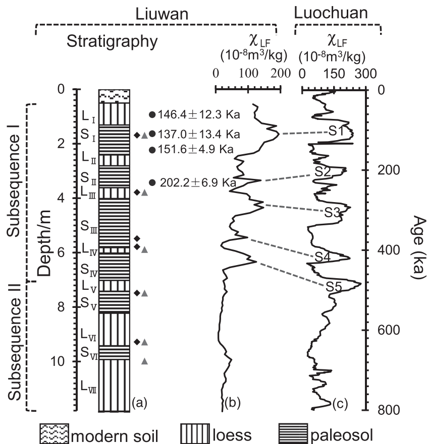
Figure 3. Pedostratigraphy (a), magnetic susceptibility (b) and their comparison with the Luochuan loess sequence (c) in the central Chinese Loess Plateau (Bloemendal & Liu 2005). Solid diamonds, triangles and circles are the locations of samples collected for high-temperature magnetic susceptibility and hysteresis loop measurements and OSL analyses.
