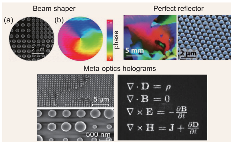
Figure 3. Examples of dielectric metasurfaces. Top left: (a), (b) SEM image of a fabricated silicon Huygens' metasurface (that transforms a Gaussian beam into a vortex beam), with a retrieved phase of the generated vortex beam, respectively [48]. Top right: Optical microscope and SEM images of a metasurface-based perfect reflector [53]. Bottom: SEM images of the fabricated meta-optics holograms and an experimental holographic image at 1600 nm wavelength [57].
