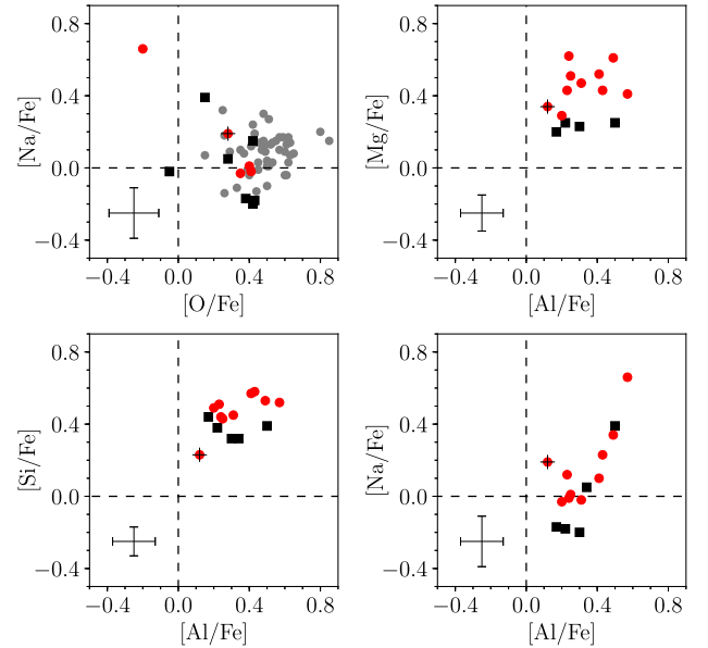
Figure 8. Red circles: this work, with a black cross over a red circle marking star b6 due to its lower SNR. Black squares: stars 1 to 7 as computed by RA16. Grey circles: HB stars from NGC 6723 (Gratton et al. 2015). Typical \sigma uncertainties by species for this work are presented on the lower left of each panel.
