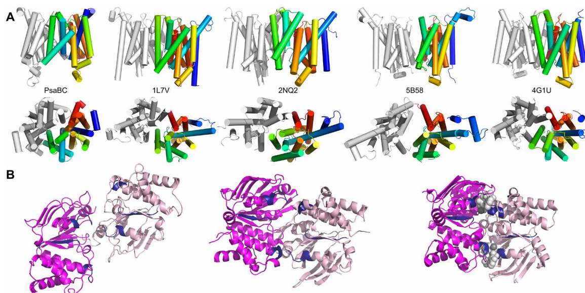
Fig. 3. Comparison of the F^{100S} PsaB 2 C 2 structure with those of other permeases. (A) The structures of the TMDs of F^{100S} PsaB 2 C 2 and homologs are shown in cartoon representations, with one monomer colored gray and the other from blue at the N terminus to red at the C terminus. Helices are shown as cylinders. The bottom representation is a rotation of the top view by 90°, parallel to the membrane plane. From left to right: F^{100S} PsaC (this work), BtuC (32) ( E. coli ; PDB 1L7V), MolA (20) ( H. influenzae ; PDB 2NQ2), BhuU (19) ( B. cenocepacia ; PDB 5B58), and HmuU (12) ( Yersinia pestis ; PDB 4G1U). (B) Alignment of the NBD structures. From left to right: PsaB (this work), BhuV 23 (PDB 5B58), and CbiO 35 ( R. capsulatus ; PDB 5X40). In all panels, the NBD monomers are shown in magenta and light pink, and the ABC, Walker B, and P loop residues are highlighted in dark blue. For the CbiO structure, the bound nucleotide and magnesium ion are shown as gray spheres.
