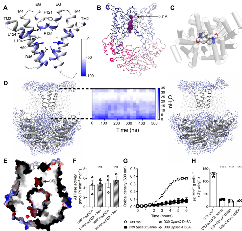
Fig. 2. The \text{Mn}^{2+} translocation pathway in PsaBC. (A) Structural elements composing the translocation pathway with Phe 121 , Leu 124 , Phe 125 , Leu 104 , His 50 , and Asp 46 shown as sticks. Residue conservation (65 TMDs from 52 characterized transporters; fig. S6) mapped to PsaC (<50%, white; 50 to 100%, white to blue). (B) Volume of the \text{F}_{1005} PsaB 2 C 2 translocation pathway visualized in purple; arrow denotes 0.7-Å closure. (C) \pi - \pi stacking between Phe 121 and Phe 125 . (D) MD analysis of WT PsaB 2 C 2 in a solvated membrane ( 8 \times 500 -ns simulations). Representative starting (left) and final (right) frames with time-dependent water occupancy displayed as a heat matrix (middle) aligned to the structure (dashed lines). PsaB (gray cartoon), PsaC (TM2 and TM4; black ribbons), and water molecules (blue sticks). (E) Representation of PsaB 2 C 2 with negatively charged surfaces in red, positive in blue, and uncharged in white. Cutaway reveals the CS (indicated by arrow). (F) ATPase activity of reconstituted \text{D}^{46\text{A}} PsaBCA and \text{H}^{50\text{A}} PsaBCA in the presence or absence of \text{Mn}^{2+} . Data represent means ( \pm SEM) from three independent experiments. (G) Growth of WT S. pneumoniae (D39 rpsL + ) and the mutant strains in \text{Mn}^{2+} -limited medium. Data represent means ( \pm SD) absorbance measurements from three independent experiments. (H) \text{Mn}^{2+} accumulation of S. pneumoniae strains in \text{Mn}^{2+} -limited media. Data represent means ( \pm SD) from three independent experiments. Statistical significance was determined by one-way ANOVA with Tukey posttest [ P > 0.05 , not significant (ns); **** P < 0.0001 ].
