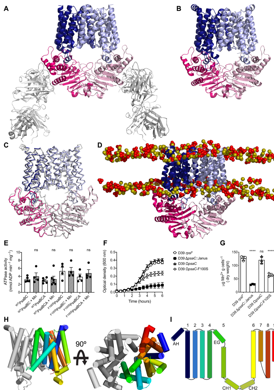
Fig. 1. Structure and activity of the PsaBC transporter. (A) F^{100S} PsaB 2 C 2 -Fab 2 complex (space group C222 1 ; PsaC, blue and lavender; PsaB, hot and light pink; Fabs, gray). (B) F^{100S} PsaB 2 C 2 structure [space group P1; colored as in (A)]. (C) Superposition of F^{100S} PsaB 2 C 2 -Fab 2 and F^{100S} PsaB 2 C 2 structures [ F^{100S} PsaB 2 C 2 -Fab 2 colored as in (B); F^{100S} PsaB 2 C 2 in gray]. Fabs omitted for clarity. (D) MD snapshot of W^T PsaB 2 C 2 [colored as in (A)] in a PG and CDL membrane. Headgroups of lipid species (PG, yellow; CDL species, orange) are shown as spheres with tails hidden. (E) ATPase activity of reconstituted W^T PsaBC and F^{100S} PsaBC with Mn 2+ and/or PsaA. Data represent means (± SEM) from at least four independent experiments. (F) Growth of WT S. pneumoniae (D39 rpsI + ), the isogenic mutant, and complemented strains (Δ) in Mn 2+ -limited media. Data represent means (± SD) absorbance measurements from three independent experiments. (G) Mn 2+ accumulation of S. pneumoniae strains in Mn 2+ -limited media. Data represent means (± SD) from three independent experiments. Statistical significance was determined by one-way analysis of variance (ANOVA) with Tukey posttest ( P > 0.05 , not significant (ns); **** P < 0.0001 ). (H) PsaC (from F^{100S} PsaB 2 C 2 ) with helices represented as cylinders. One monomer is colored gray, the other is colored from blue (N terminus) to red (C terminus). (I) Topology of PsaC monomers with helices numbered (AH, amphipathic helix; EG, extracellular gate; CH, coupling helix). Colors correspond to (H).
