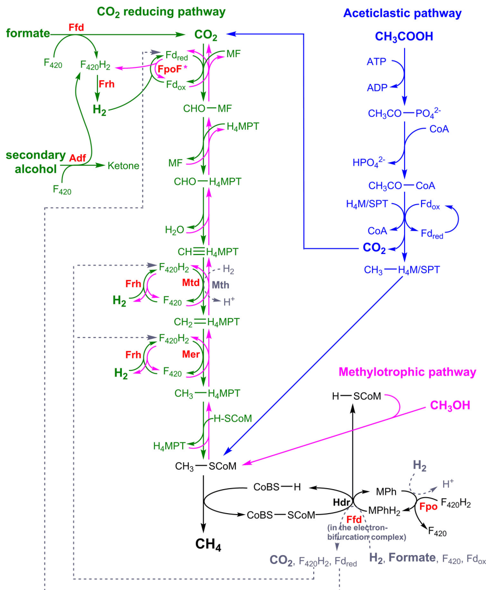
FIG 7 \text{CO}_2 -reducing (green), methylotrophic (pink), and aceticlastic (blue) pathways of methanogenesis. The routes for energy generation from \text{H}_2/\text{CO}_2 , formate, secondary alcohols, methanol, and acetate are shown. Processes common to all pathways are shown in black, and dashed arrows in gray show alternative pathways. \text{F}_{420} -dependent oxidoreductases are highlighted in red and catalyze both forward and reverse reactions, except for \text{FpoF} which is known to catalyze only \text{F}_{420}\text{H}_2 reoxidation. Abbreviations: \text{F}_{\text{red/ox}} , reduced/oxidized ferredoxin; MF, methanofuran; \text{H}_4\text{MPT} , tetrahydromethanopterin; \text{H}_4\text{SPT} , tetrahydrosarcinapterin; \text{H-SCoM} , 2-mercaptoethanesulfonate (reduced coenzyme M); \text{CoBS-H} , N-7-mercaptoheptanoylthreonine phosphate (reduced coenzyme B); \text{MPh}/\text{MPhH}_2 , reduced/oxidized methanophenazine.
