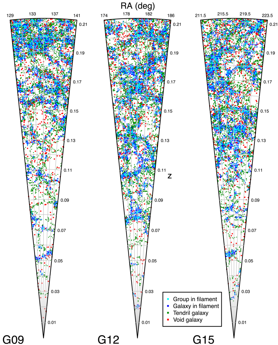
Figure 9. Galaxy distribution in the three GAMA regions, colour coded according to their environment, with groups in filaments, galaxies in tendrils and void galaxies shown in cyan, blue, green and red, respectively. Groups and galaxies near them form the bulky complexes of large-scale structure, tendrils spreading from them in filamentary structures into voids, which seem to be populated by galaxies that appear to be almost uniformly distributed on large scales.
