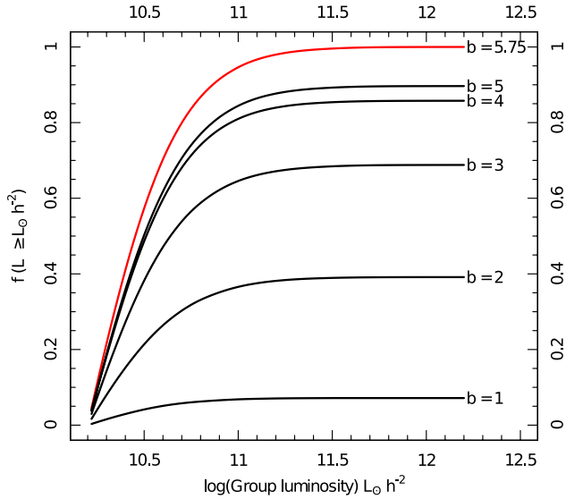
Figure 6. Cumulative fraction of groups in filaments as a function of their total r -band group luminosity, shown for different maximum edge lengths in the MST (given by b ). As b decreases we begin to only construct filaments between pairs of groups that are in extreme close proximity, and the fraction of high-mass groups in filaments drops to 0. Naturally, if we raised b to a much higher value all groups would be in a single giant filament. We therefore select the minimum value for b at which 90 per cent or more of galaxies with L_{\text{Group}} \geq 10^{11} L_{\odot} h^{-2} are in filaments, or in other words, f(L_{\text{Group}} \geq 10^{11} L_{\odot} h^{-2}) \geq 90 per cent.
