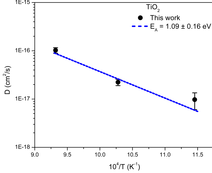
Figure 6: Arrhenius plot for three annealing temperatures.
