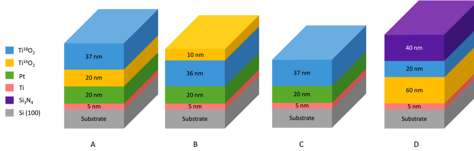
Figure 1: Sketch of samples studied for oxygen self diffusion in \text{TiO}_2 . The oxygen profile and the electrical behavior of A, B and C were analyzed. Sample D was produced for diffusion studies.
