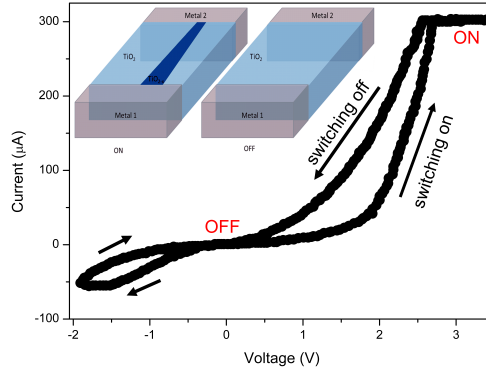
Figure 2: Electric measurements of sample C after deposition of an aluminum electrode with thickness of 400 nm. The inset shows a sketch of the formation of a filament inside \text{TiO}_2 , which causes the change in resistance.
