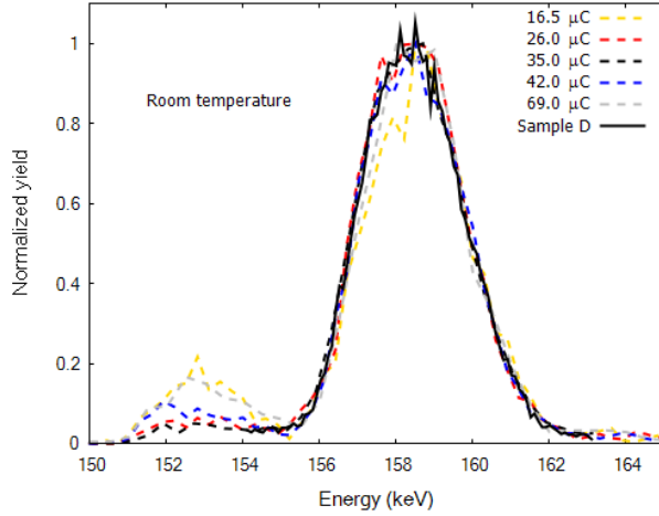
Figure 4: Experimental excitation curves for protons in non-annealed sample similar to sample D for different fluences ( 1\mu C = 2.5 \times 10^{13} atoms \text{cm}^{-2} ). The excitation curve for the non-annealed sample D used for the diffusion experiments is also shown.
