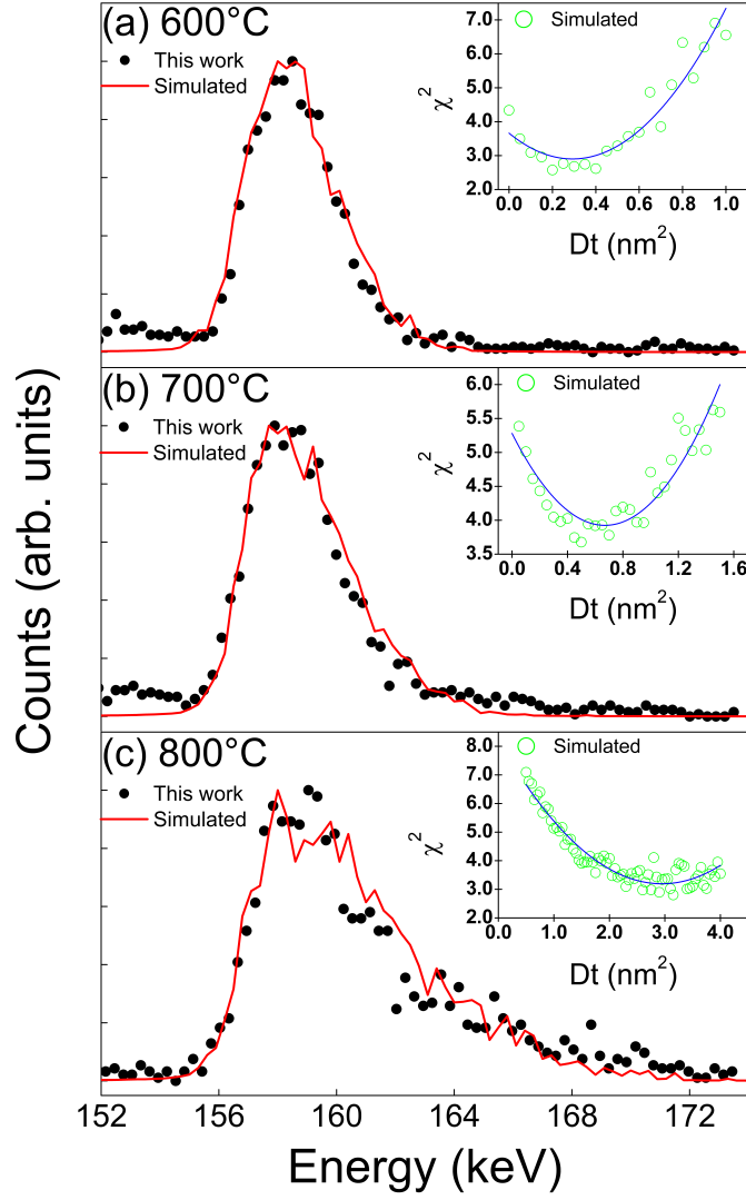
Figure 5: Experimental excitation curves and fitting for sample D annealed at (a) 600 °C, (b) 700 °C and (c) 800 °C. The insets show the corresponding \chi^2 values of the fit versus Dt value assumed for each simulation.
