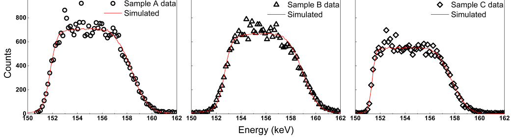
Figure 3: Excitation curves of ^{18}\text{O} measured with nuclear reaction ^{18}\text{O}(\text{p}, \alpha)^{15}\text{N} for samples A, B and C.
