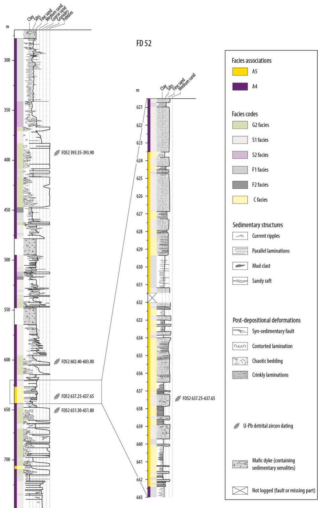
Fig. 10. Sedimentological log of the drill core intersecting the Igarapé Bahia Group. Facies codes: Table 3. Facies association: Table 4. The upper part of the drill core intercepts another formation (Appendix 1).
