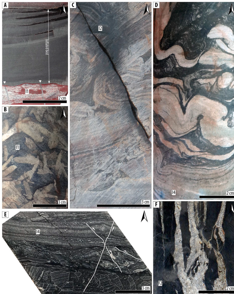
Fig. 7. Syn-to post-depositional deformations, diagenetic and metamorphic features in the Carajás Formation. Arrows point to the stratigraphic top. Facies codes: Table 3. A. Sample FD55 351.90. Jaspilitic BIF comprising a late diagenetic inflated bed composed of magnetite with small veins rooted in the inflated bed (white triangles) crosscutting the underlying BIF. B. Sample FD354 242.20. Large secondary minerals in a jaspilitic BIF. C. Sample S11D214 449.00. Chert displaying folded layers and a few clasts, attesting for a ductile to brittle deformation attributed to slumping processes. D. Sample FD365 340.80. Highly contorted lamination in carbonate BIF resulting from the loading of dense Fe-rich layers onto carbonate beds. E. Sample FD365 262.20. Carbonate BIF showing intraformational angular clasts along a slip surface. Syn-sedimentary faults crosscut both intraformational clasts and carbonate BIF. Two erosion surfaces are present above the intraformational angular clasts. F. Sample S11D214 323.10. Injectite in black shales.
