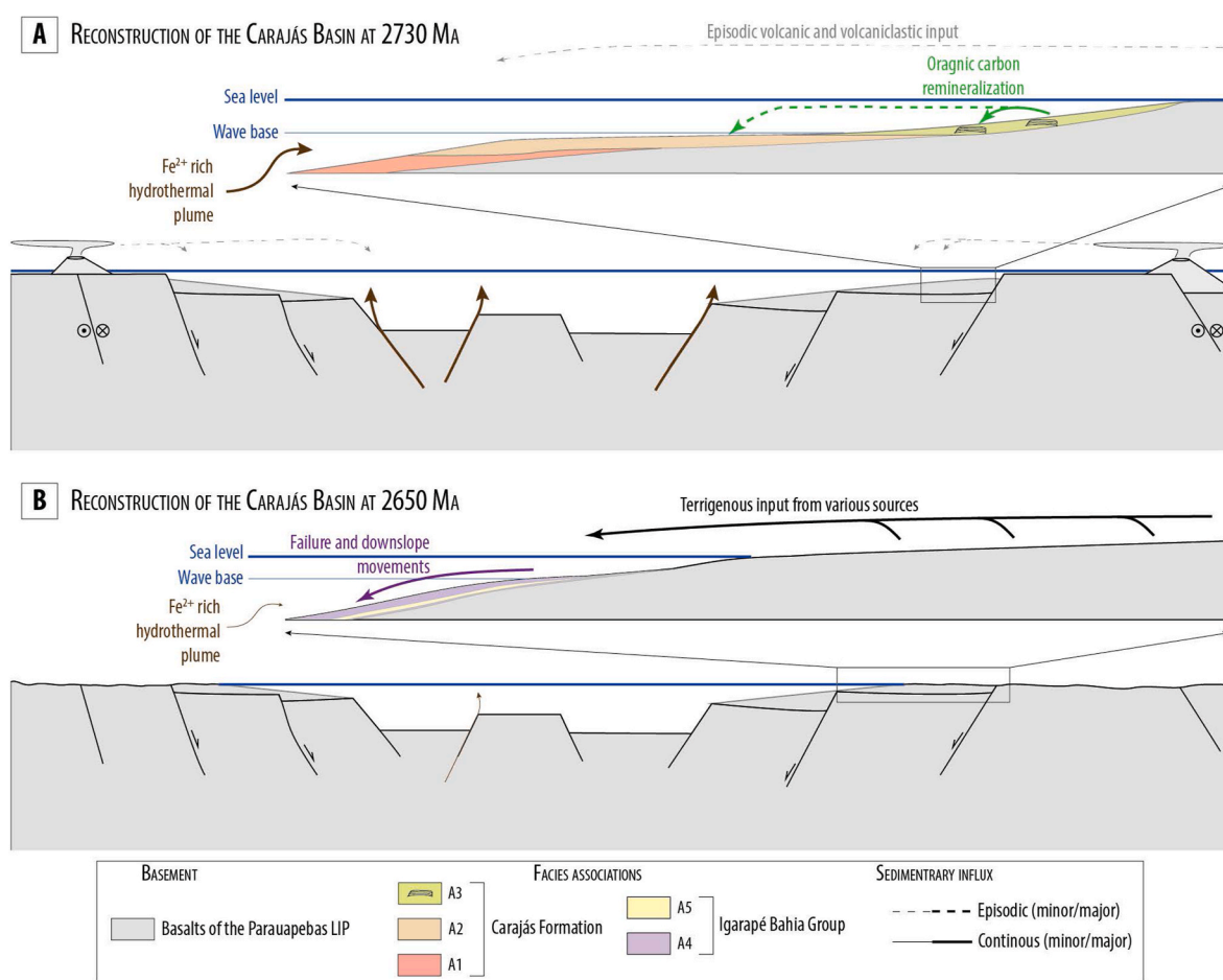
Fig. 14. Schematic cross-sections of the Carajás Basin during the Neoarchean. A. Paleoenvironmental and tectonic settings of the Carajás Basin during the deposition of the Carajás Formation, at ca. 2730 Ma. B. Paleoenvironmental and tectonic settings of the Carajás Basin during the deposition of the Igarapé Bahia Group at ca. 2650 Ma.
