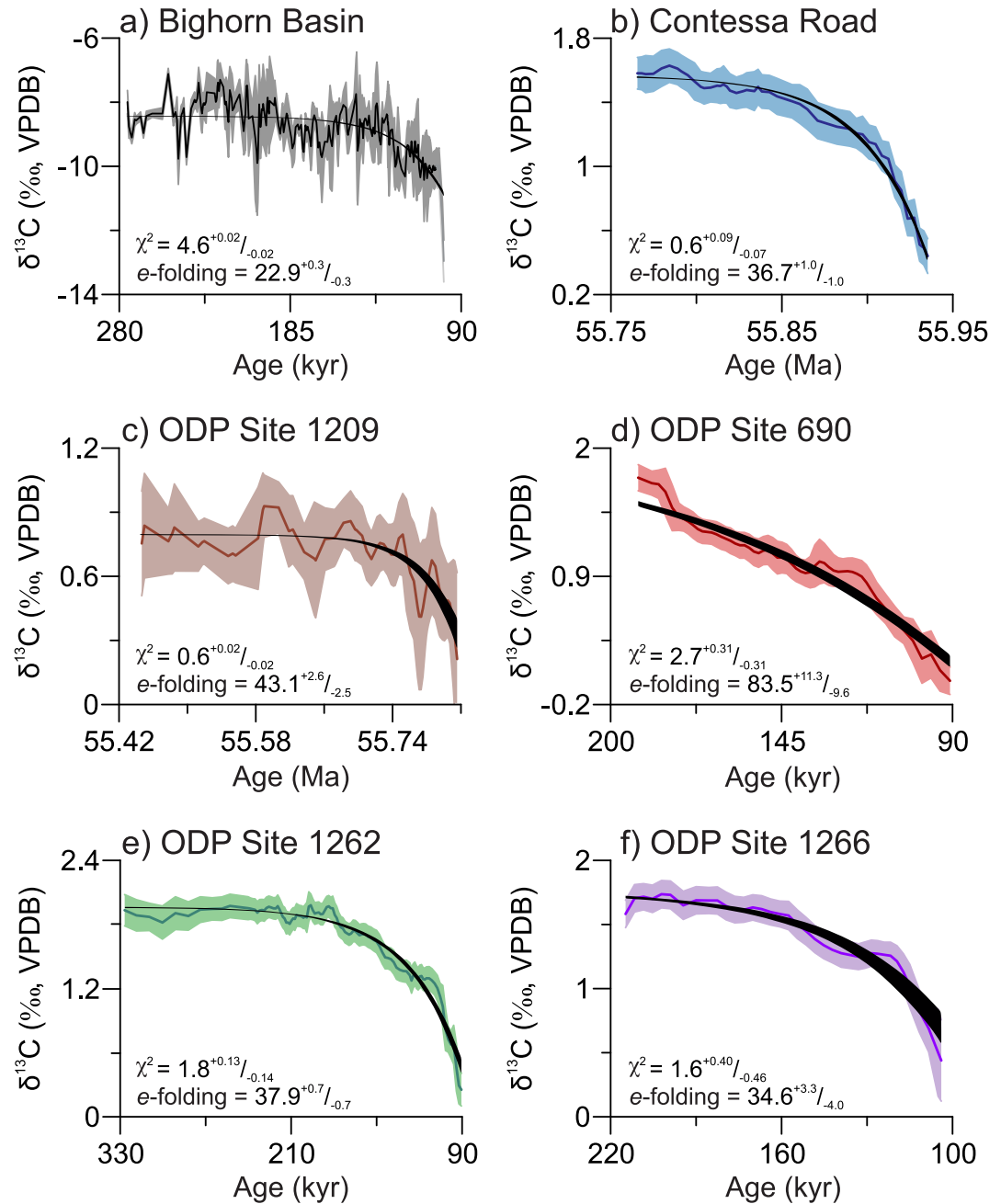
Figure 2. Exponential decay functions presented in terms of their 95% confidence intervals (black) for the PETM CIE recovery interval at (a) Bighorn Basin, (b) Contessa Road, (c) ODP Site 1209, (d) ODP Site 690, (e) ODP Site 1262, and (f) ODP Site 1266. Background \delta^{13}\text{C} records are indicated in dark (mean) and light shading ( \pm 2 standard error (2SE)). Age scales are based on the PETM CIE recovery onset according to the age model for each studied section.
