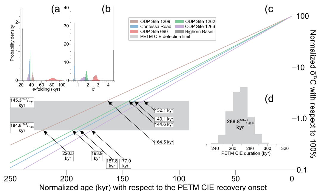
Figure 3. Probability density distributions for (a) e -folding and (b) \chi^2 values of exponential decay functions from each studied \delta^{13}\text{C} record. (c) Modeled exponential decay functions for normalized \delta^{13}\text{C} values (100%) that decay at rates defined by e -folding timescales (ODP Site 1209 = 43.1 kyr, ODP Site 1262 = 37.9 kyr, Contessa Road = 36.7 kyr and ODP Site 1266 = 34.6 kyr). The PETM CIE detection limit is indicated by a gray rectangle that is limited by the 0.6%–2.2% interval (see Supporting Information S1). Durations in white rectangles represent PETM CIE recovery duration estimates for each section, while values in bold letters represent probabilistic-based PETM CIE recovery duration estimates for each PETM CIE detection boundary. (d) Probability density distribution for the PETM CIE duration. The median and 95% confidence interval of this distribution are indicated as our probabilistic-based PETM CIE duration estimate.
