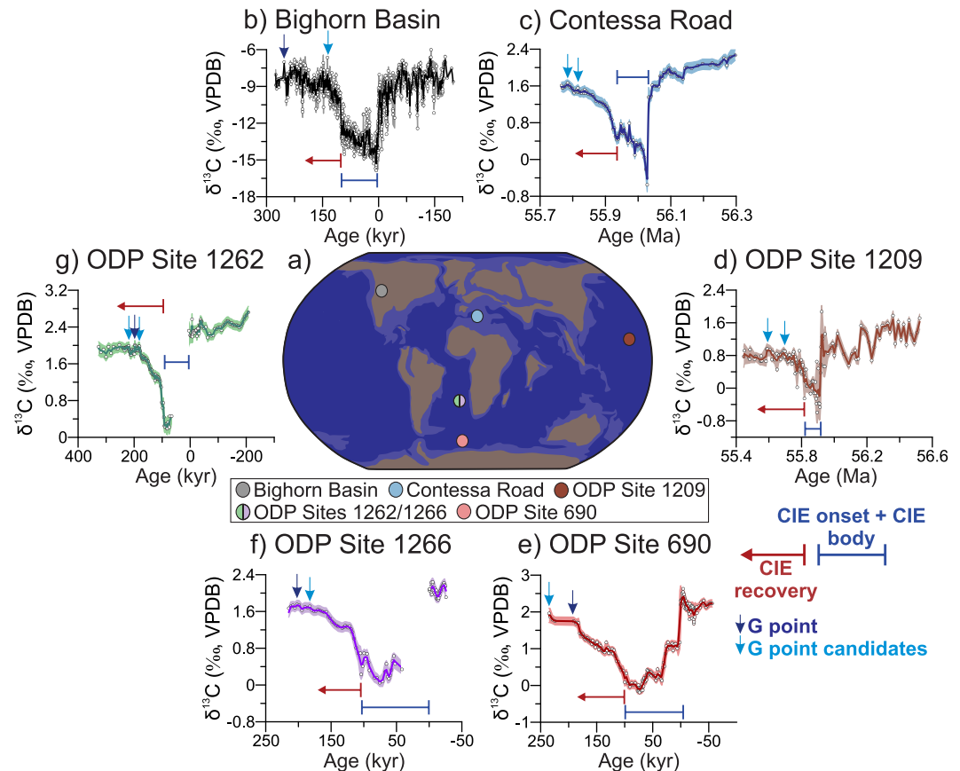
Figure 1. (a) Paleogeographic reconstruction at ~56 Ma (Pogge von Strandmann et al., 2021) with locations of the studied Paleocene-Eocene Thermal Maximum (PETM) \delta^{13}\text{C} records from (b) Bighorn Basin, (c) Contessa Road, (d) ODP Site 1209, (e) ODP Site 690, (f) ODP Site 1266, and (g) ODP Site 1262. White dots represent raw data; continuous dark lines indicate the mean \delta^{13}\text{C} , with envelopes surrounding these lines indicating \pm 2 standard error (2SE) intervals. Horizontal lines for each record represent different PETM carbon isotope excursion (CIE) phases. Dark- and sky-blue arrows indicate the G point according to previous studies (van der Meulen et al., 2020; Westerhold, Röhl, Wilkens, et al., 2018) and similar \delta^{13}\text{C} inflections referred to as G point candidates, respectively.
