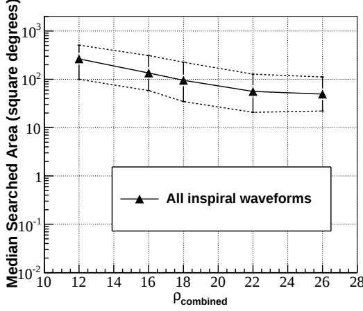
Fig. 5. Plots of uncertainty region sizes for the MBTA pipeline as a function of combined SNR ( \rho_{\text{combined}} ). The solid line with symbols represents the median (50%) performance, while the upper and lower dashed lines show the 75% and 25% quartile values. The expected detection threshold is around \rho_{\text{combined}} \sim 12 .
