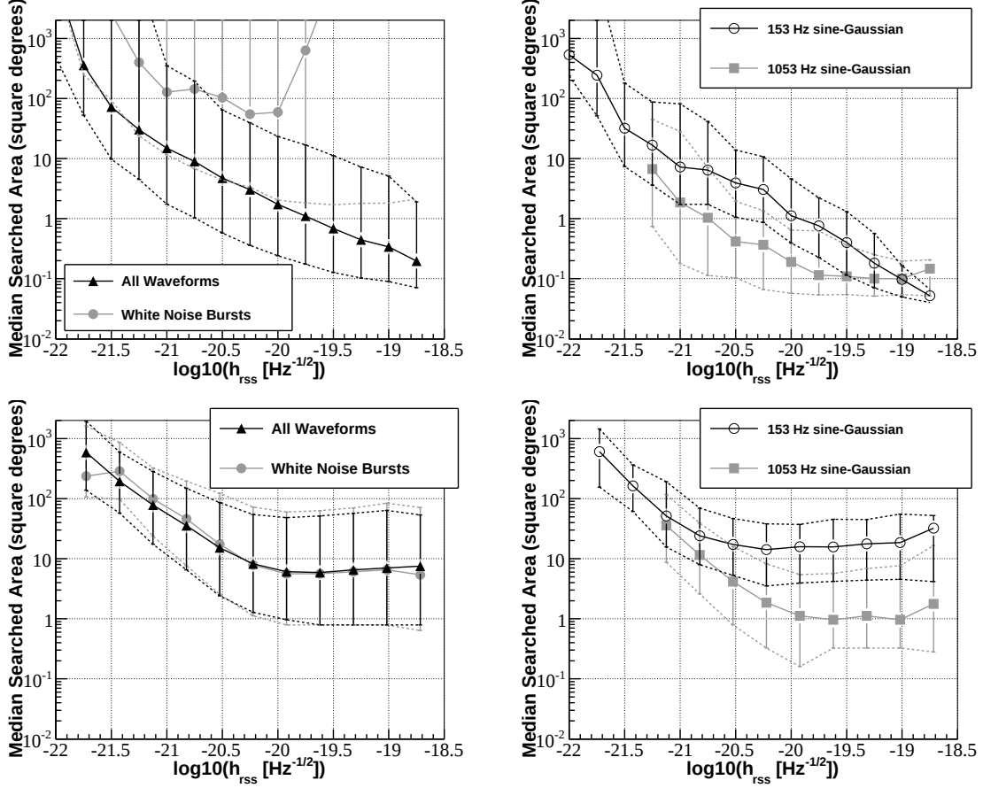
Fig. 4. Plots of typical uncertainty region sizes for the Omega (top) and unconstrained cWB (bottom) pipelines, as a function of GW strain amplitude at Earth, for various waveform types. The “searched area” is the area of the skymap with a likelihood value greater than the likelihood value at the true source location before the galaxy catalog is used to further limit the search region. The solid line with symbols represents the median (50%) performance, while the upper and lower dashed lines show the 75% and 25% quartile values. Near the detection threshold ( h_{\text{rss}} \sim 10^{-21} \text{ Hz}^{-1/2} ), uncertainty regions are typically between 10 and 100 square degrees. The Omega pipeline performs poorly on white noise bursts but exceptionally well on sine-Gaussians because it is designed to identify signals that are well-localized in frequency space.
