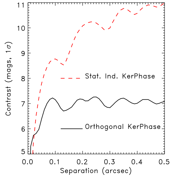
Figure 3. The effect of photon noise on kernel phase detections, based on a simulated photon-limited image with 10^6 photons taken with the unobstructed Keck telescope in the Lp filter. The decreased number of photons far from the PSF core means that kernel phases sensitive to these spatial locations have smaller errors, increasing the achievable contrast. Although the kernel phases in each situation are equivalent, the uncertainties are not equivalent and would require a full covariance matrix in the case of the orthogonal kernel phase.
