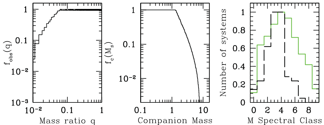
Figure 5. From left to right: mass ratio distribution, companion mass distribution f_c(M_s) and spectral class distribution of M dwarf companions for a pairing of the type given by equation (4) with \beta = 0 . The panel on the right shows the normalized SDSS M dwarf distribution of wide white dwarf–M dwarf binaries (dashed line), while the solid line shows the model prediction for the distribution of M dwarfs.
