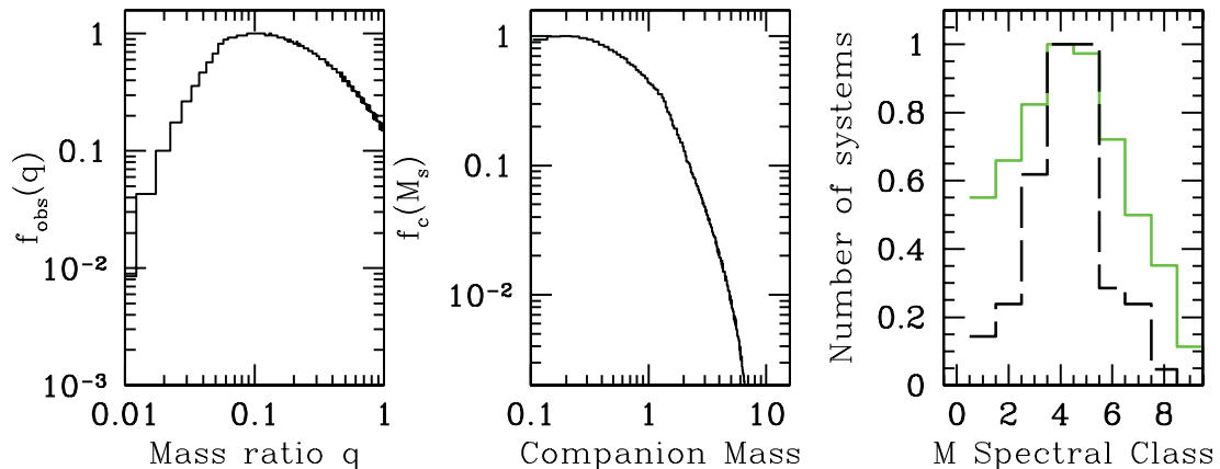
Figure 4. From left to right: mass ratio distribution, companion mass distribution f_c(M_s) and spectral class distribution of M dwarf companions for a pairing of the type given by equation (3) with \sigma = 0.4 and k = 0.5 . The panel on the right shows the normalized SDSS M dwarf distribution of wide white dwarf–M dwarf binaries (dashed line), while the solid line shows the model prediction for the distribution of M dwarfs.
