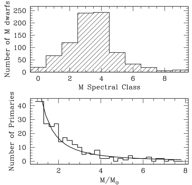
Figure 1. Top panel: spectral class of M dwarf companions to white dwarfs in the wide binaries of Rebassa-Mansergas et al. (2010). Bottom panel: mass distribution of white dwarf progenitors after a final-to-initial mass relationship has been applied to the white dwarfs in the wide binaries in Rebassa-Mansergas et al. (2010) (see text for details). Solid curve: best power-law fit with index \alpha = -1.95 \pm 0.14 .
