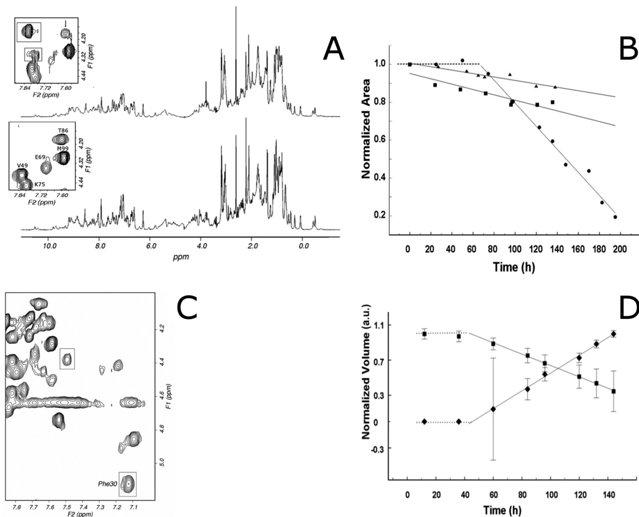
FIGURE 2. A, 500 MHz 1 H NMR spectra of an ordinary sample of R3Aβ 2 m (~0.9 mM, 310 K, pH 6.6) in the absence (lower trace) and presence (upper trace) of an equimolar amount of αB-crystallin subunit. The only apparent consequence of the sHsp addition is a general broadening, with conservation of the spectral pattern of R3Aβ 2 m. The insets show a portion of the H N -H α connectivity (fingerprint) region of the corresponding two-dimensional TOCSY spectra. The boxed cross-peaks arise from the unstructured and flexible C-terminal extension of αB-crystallin. Only this region of 12 amino acids is present in the spectrum by virtue of its fast local tumbling as opposed to the extremely slow overall motion of αB-crystallin oligomer (~650 kDa) that causes the extreme broadening of other resonances (34–36, 60). Assignments are indicated for R3Aβ 2 m NH to α-CH cross-peaks (12, 19). Arrows mark visibly attenuated R3Aβ 2 m connectivities for Q69 and T86. B, time evolution of the upfield-shifted methyl resonance (L23 δ 1 CH 3 ), which is diagnostic for the correctly folded species, of an ordinary sample of R3Aβ 2 m obtained from 500 MHz 1 H one-dimensional NMR spectra, in the absence (circles) and in the presence of αB-crystallin at equimolar (squares) or halved concentration (triangles) with respect to R3Aβ 2 m. The average rate of loss of signal intensity was (5.6 \pm 0.5) \times 10^{-3} \text{ h}^{-1} in the absence of αB-crystallin and (1.5 \pm 0.5) \times 10^{-3} or (1.8 \pm 0.5) \times 10^{-3} \text{ h}^{-1} for 1:2 or 1:1 αB-crystallin/R3Aβ 2 m mixtures, respectively. The errors on the rates were estimated by considering the deviations obtained when assessments were made using absolute resonance amplitudes rather than self-normalized values (53) to account for the uncertainties introduced by the scaling procedure. Generally speaking, such uncertainties arise when resonances with smaller linewidths overlap pre-existing signals, as well as from the general linewidth increase upon addition of αB-crystallin. C, two-dimensional TOCSY fingerprint details obtained from an 82-h-old solution of R3Aβ 2 m (0.8 mM, 310 K, pH 6.6). The boxed cross-peaks represent the NH-αCH connectivities whose time evolution is displayed in D, respectively, from Phe-30, in the folded protein, and from an unknown residue, in the unfolded soluble species. D, time dependence of the two-dimensional TOCSY cross-peak amplitudes of C (Phe-30 = squares, unassigned = diamonds). In the absence of αB-crystallin, the evolution of the resolved fingerprint cross-peaks showed typically a similar trend as that obtained by considering the evolution of the resolved methyl resonances in one-dimensional 1 H spectra (B). Indeed, the slope of the decreasing Phe-30 cross-peak amplitude is -5.9 \times 10^{-3} \text{ h}^{-1} , i.e. in absolute value the same, within the experimental error, as the slope of the unknown cross-peak intensity.
