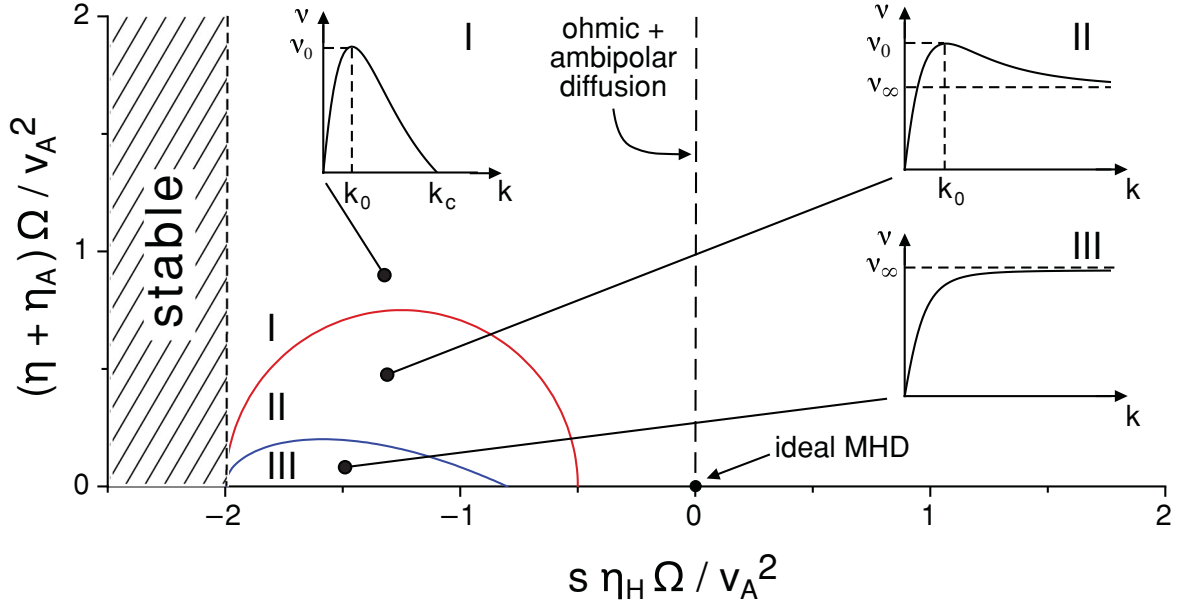
Figure 5. Schematic dependence of the behaviour of the MRI on the Hall and Pedersen (Ohm+ambipolar) diffusivities, \eta_H and \eta_P , for an initial magnetic field sB_z\hat{z} in a Keplerian disc, where s = \pm 1 is the sign of B_z . The field is assumed to be weak so that stratification can be neglected. Physical values of the Pedersen conductivity \eta_P are non-negative, and there are no unstable modes for Hall diffusivities s\eta_H\Omega/v_A^2 \leq -2 . The unstable region s\eta_H\Omega/v_A^2 > -2 is subdivided according to the dependence of the growth rate on wavenumber k , which is sketched in the insets labelled I–III. In region I (outside the red locus given by equation B11), wavenumbers less than a cut-off k_c are unstable, with the maximum growth rate v_0 attained at k_0 (see equations B12, B13 and B14). Between the red and blue loci (region II), all wavenumbers are unstable, with the maximum growth rate still occurring at finite wavenumber. Within the blue locus given by equation (B15) (region III), all wavenumbers are unstable and the maximum growth rate is approached asymptotically as k \rightarrow \infty .
