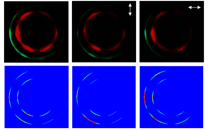
FIG. 2. (Color online) Experimentally recorded (top row) and theoretically predicted (bottom row) Čerenkov harmonic rings without analyzer and with vertical analyzer and with horizontal analyzer (from left to right). The polarization angle of the fundamental wave is \gamma=30^\circ .
