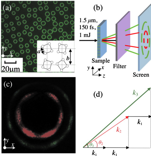
FIG. 1. (Color online) (a) The domain pattern imaged by the scanning SHG microscopy with the inset illustrating the creation of the structure. (b) Schematic of the experiment. (c) The observed Čerenkov SH and TH rings. The fundamental wave is linearly polarized along x -axis ( \gamma=0 ). (d) The PM diagram of Čerenkov THG.
