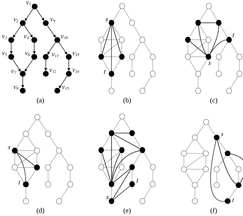
Figure 6: Some examples of contaminated sets (solid nodes) that are incident to edges added (dashed) by Algorithm (3) for different candidate edge additions ( s \rightarrow t ) to the Bayesian network shown in (a). In (b), (c), (d), and (e) the treewidth is increased by one; In (f) the treewidth does not change.
