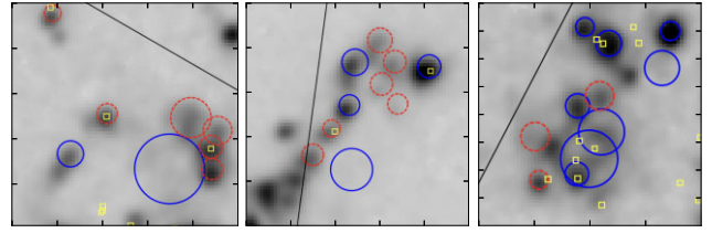
Figure 4. Spatial distribution of Class 4 sources (yellow boxes), orphan H II regions (red dashed circles), and populated H II regions (blue circles), overlaid on the H \alpha map obtained from the SIGNALS survey. The black outline indicates the FoV defined in Section 2.2. Class 4 sources are seen associated with both orphan and populated H II regions. These Class 4 sources and H II regions are, based on their locations relative to orphan H II regions, possibly associated with them.
