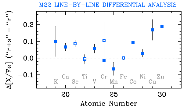
Figure 2. Differences in the mean abundances between the three r -only stars and the three r+s stars as a function of atomic number for K through Zn. Solid squares indicate neutral species, and open squares indicate singly ionized species. The dotted line indicates zero difference.
