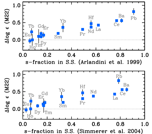
Figure 8. Differences in the mean abundances between the r -only group and the r+s group as a function of the s -fraction of each element in the S.S. The top panel shows the s -fraction as calculated from the average yields of the 1.5 and 3.0 M_{\odot} stellar models at [\text{Fe}/\text{H}] = -0.3 of Arlandini et al. (1999), including the contribution of low-metallicity AGB stars to the S.S. Pb as derived by Travaglio et al. (2001). The bottom panel shows the s -fraction as calculated by the classical method (Simmerer et al. 2004). The dotted lines indicate zero difference.
