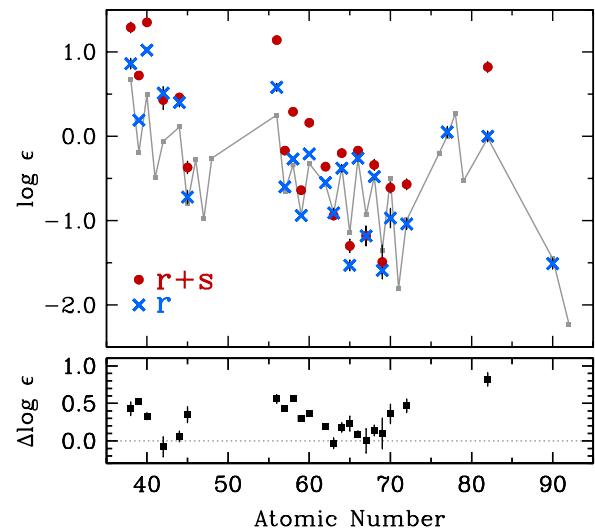
Figure 4. Top panel: the mean logarithmic abundances for the three r -only stars (blue crosses) and the three r+s stars (red circles) as a function of atomic number. The gray line and small gray squares illustrate the abundances in the r -process standard star BD + 17 3248 (Cowan et al. 2002, 2005; Sneden et al. 2009; Roederer et al. 2010b). Pb has not been detected in BD + 17 3248, so we instead show the predicted Pb/Eu ratio based on the average Pb/Eu observed in Figure 3 of Roederer et al. (2010a). The BD + 17 3248 abundance pattern has been normalized to the Eu abundance. Bottom panel: the differences in these mean abundances. The dotted line indicates zero difference.
