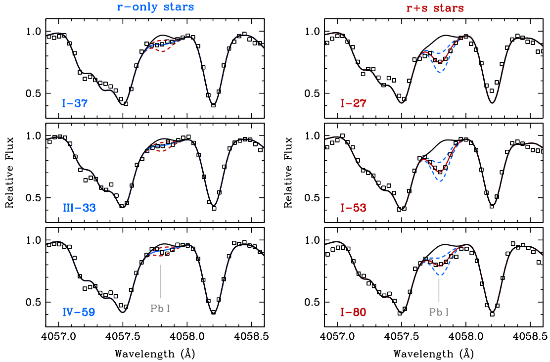
Figure 1. Comparison of observed (open squares) and synthetic (lines) spectra around the Pb I 4057.8 Å line. The left panels show the three r -only stars, and the right panels show the three r+s stars. The solid colored line (left panels, blue; right panels, red) indicates the best-fit abundance, the dashed lines indicate variations in the best-fit abundance by 0.3 dex, and the solid black line indicates a synthesis with no Pb I present.
