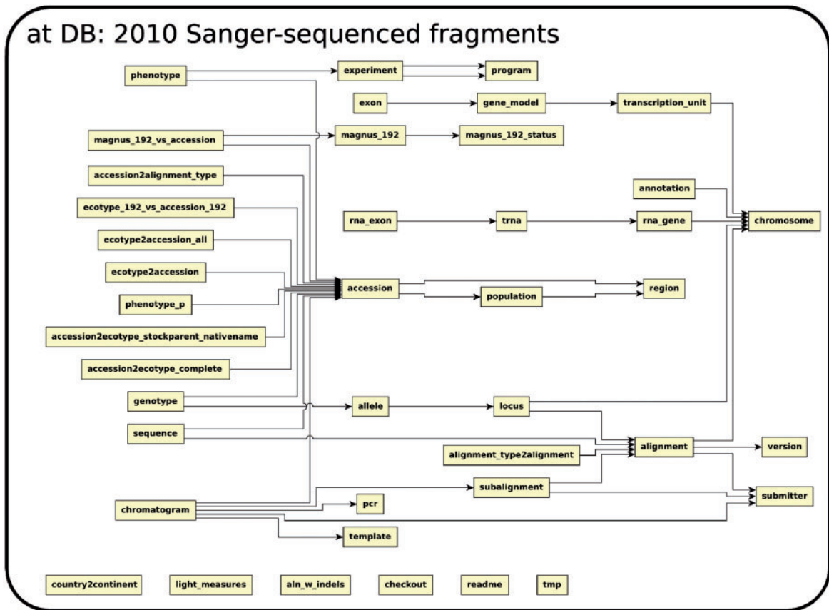
Figure 2. The relationship among tables in subdatabase at.
