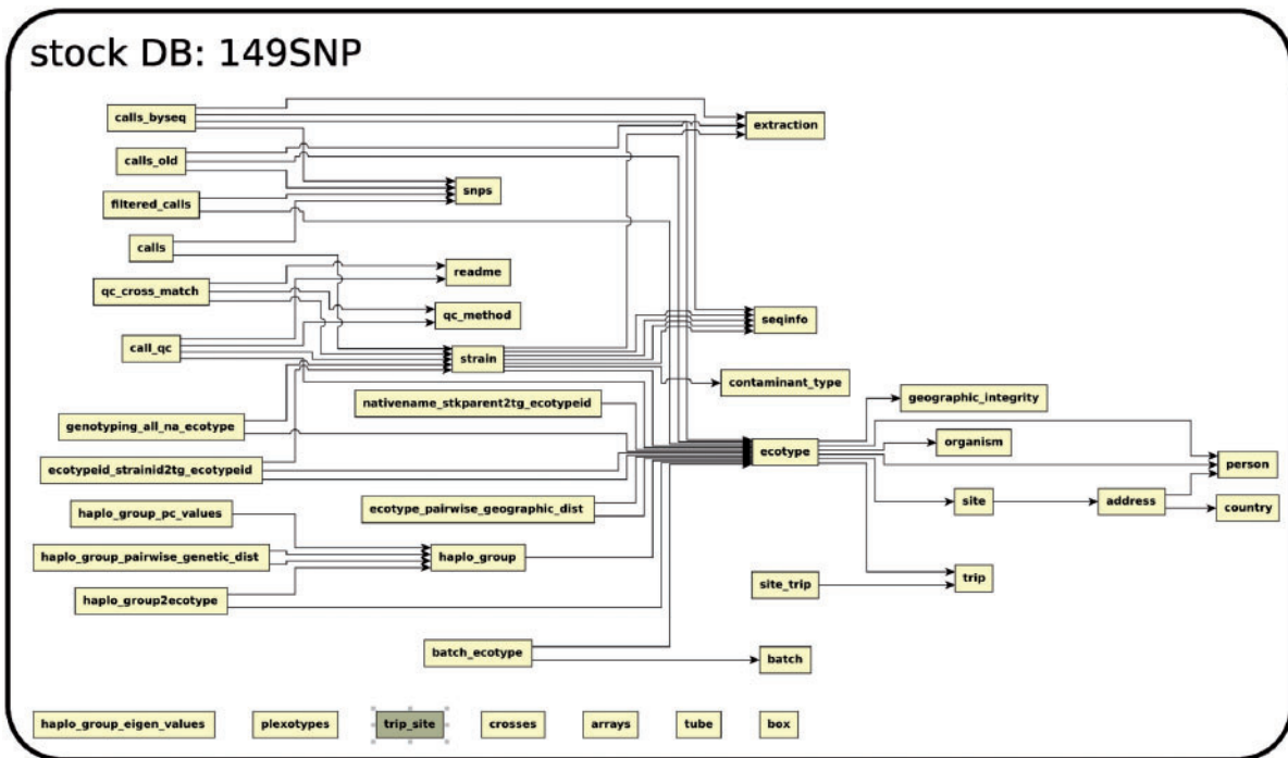
Figure 3. The relationship among tables in subdatabase stock.
