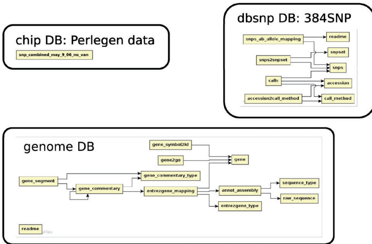
Figure 4. The relationship among tables in subdatabase chip, dbsnp and genome.
