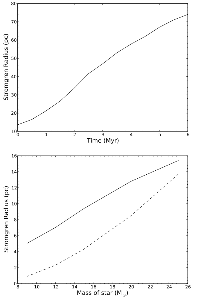
Figure 10. Top: the Strömgen radius of a 25 M_{\odot} star as a function of time. The Strömgen radius increases with time as the star removes much of the neutral gas from its environment. This creates an exclusion zone where star formation is temporarily stopped. Bottom: the Strömgen radius of a star in the initial gas density profile as a function of mass for the case of zero metallicity (dashed line) and [\text{Fe}/\text{H}] = -1.7 (solid line). The affected volume rises as a steep function of stellar mass, with the more common supernova-forming stars having a very small Strömgen radius and therefore a pre-ionization phase that can be neglected.
