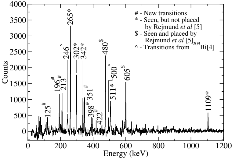
Fig. 2. Spectrum gated on the 2465 keV transition in ^{207}\text{Tl} , showing transitions above the 11/2^- isomer, as well as transitions in the ^{209}\text{Bi} partner nucleus. A number of new transitions have been seen in ^{207}\text{Tl} , and the existence of those seen by Rejmund et al. can be confirmed [5].
