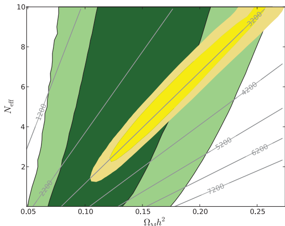
Figure 5. The constraints in the N_{\text{eff}}-\Omega_{\text{M}} h^2 plane derived from the WiggleZ measurement of the turnover scale (in green) compared to CMB COSMOMC constraints from WMAP (in yellow). The dark-shaded regions depict 68 per cent confidence intervals and the light-shaded regions depict 95 per cent confidence intervals. The grey contours depict lines of constant \Omega_{\text{M}}/\Omega_{\text{r}} = 1 + z_{\text{eq}} .
