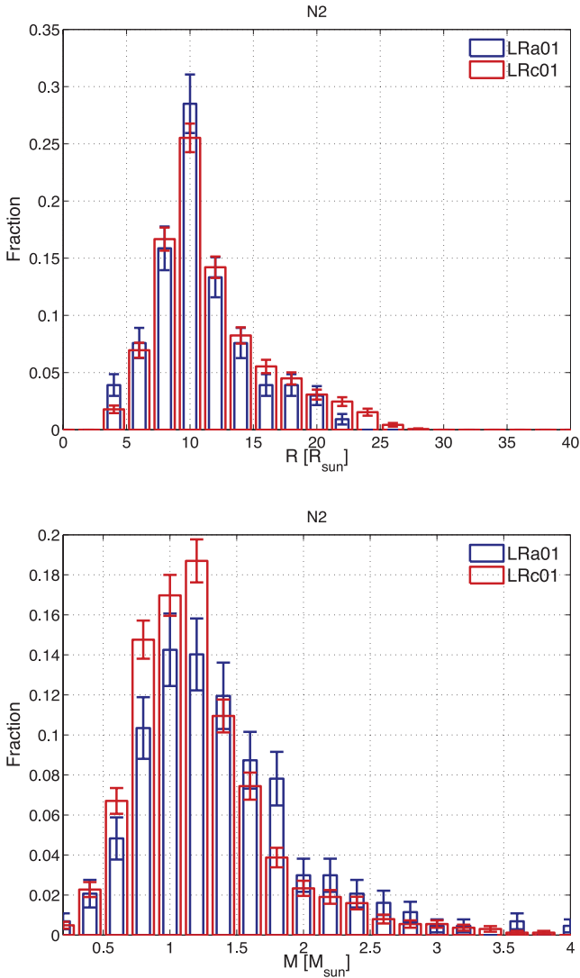
Figure 2. Radius and mass distributions of stars in LRA01 (blue) and LRC01 (red) obtained using the method described in Section 2.
