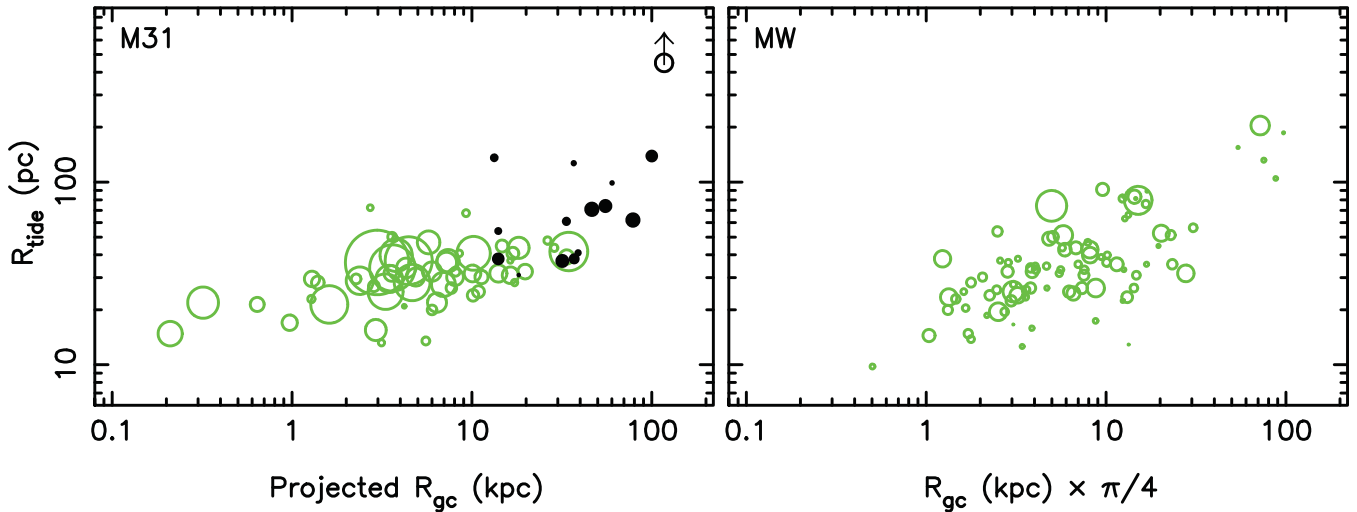
Figure 17. King-model tidal radius plotted against galactocentric distance (projected) for M31 and Milky Way globulars. Symbols and panels are same as for Fig. 15 except in this case the Strader et al. (2011) clusters are not plotted since tidal radii were not given in their paper.
