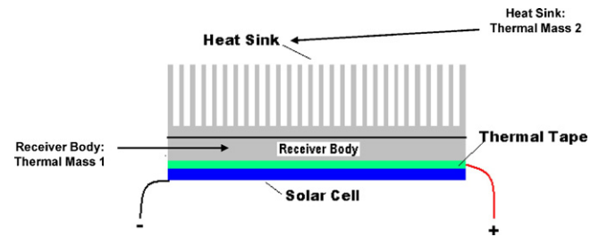
Fig. 1. Example of a passively-cooled receiver with attached heat sink.
