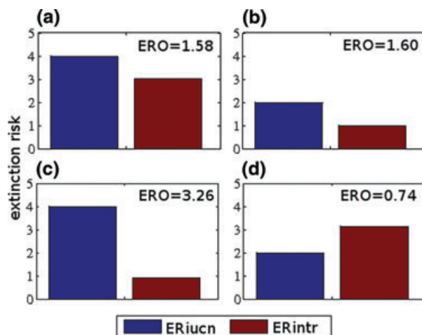
Figure 1 The ERO (Extinction risk Reduction Opportunity) components. The graph shows the current ( ER_{IUCN} ) and intrinsic ( ER_{INTR} ) extinction risk of four example species and their associated ERO values (derived from (1) in "Methods"; see Table S2 for a complete species' list). (a) The Aders' Duiker ( Cephalophus adersi ) has both a high ER_{IUCN} and a high ER_{INTR} values, resulting in a medium ERO value. (b) The Clouded Leopard ( Neofelis nebulosa ), has a both a low ER_{IUCN} and a low ER_{INTR} values, resulting in a medium ERO value. (c) The Black-spotted Cuscus ( Spilogocus rufoniger ) has a high ER_{IUCN} value and a low ER_{INTR} value, resulting a high ERO value. (d) The Andaman Spiny Shrew ( Crocidura hispida ) has a low ER_{IUCN} value and a high ER_{INTR} value, resulting a low ERO value.
