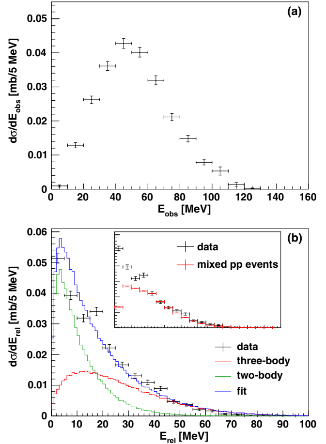
FIG. 1 (color online). (a) Energy of the dissociated ^{26}\text{Ne} + p + p fragments in their P_{c12} = 0 frame. The cross section has been corrected for the geometric efficiency of the HiRA array, as described in Ref. [11]. (b) Relative energy distribution of the two detected protons. The fractions of simulated three-body (red or dark grey) and two-body (green or light grey) kinematics events have been fitted to the data set (see text for details). The inset compares the measured relative energy distribution with that derived from mixing protons from two independent events (red or dark grey). The distribution obtained from mixed events has been scaled to the experimental two-proton relative energy distribution above 40 MeV.
