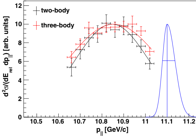
FIG. 3 (color online). Parallel momentum distribution of the ^{26}\text{Ne} residue gated on two-body (black) and three-body (red or grey) events. The two components were extracted by applying a cut on E_{\text{rel}} at the intersection of the two distributions in Fig. 1(b). Contributions from three-body events at low E_{\text{rel}} were subtracted from the two-body distribution and vice versa for the two-body events with high relative energy. The lines are Gaussian fits. The two distributions have been normalized to show the difference in width. The blue distribution illustrates the width of the momentum distribution of the incoming ^{28}\text{Mg} beam.
