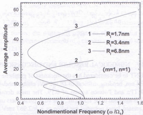
Fig. 2 Influence of large amplitudes on vibration frequency for several two-walled carbon nanotubes with different radii and the length-radius ratio L/R_0 = 10 .
