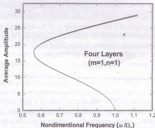
Fig. 1 Free vibrations of a four-layer carbon nanotube
