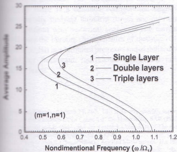
Fig. 6 Influence of amplitudes on frequency for several multi-walled carbon nanotubes with L/R_0 = 10 , R_l = 3.4 \text{ nm} .
