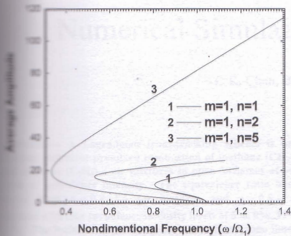
Fig. 5 Influence of large amplitudes on vibration frequency for several two-walled carbon nanotubes with different circumferential wave numbers and L/R_0 = 10 , R_l = 3.4 \text{ nm} .
