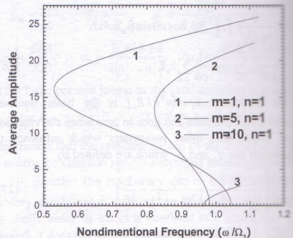
Fig. 4 Influence of large amplitudes on vibration frequency for several two-walled carbon nanotubes with different axial wave numbers and L/R_0 = 10 , R_i = 3.4\text{nm} .
