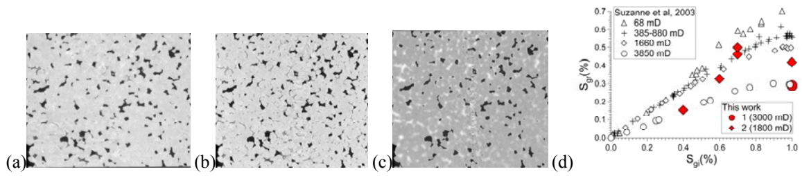
Figure 4: (a) Fontainebleau sandstone after SI into a system with initial water saturation ( S_{wi} ) = 30% (b) SI into S_{wi} = 30% (repeat), (c) SI into S_{wi} = 0%, (d) Graph displaying data from Suzanne et al, 2003, with overlaid data from the above runs.
