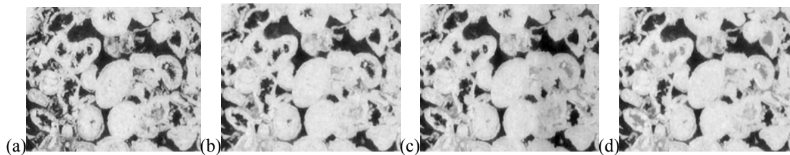
Figure 6: Subset of 3D \mu -CT image of reservoir carbonate of size 1.35x1.05 mm in size (450 x 350 pixels, at 3 microns per pixel); (a) dry sample; (b) registered slice after SI at S_{wi}=0\% ; (c) registered slice after SI at S_{wi} \sim 40\% ; (d) registered slice after SI at S_{wi} \sim 50\% .
