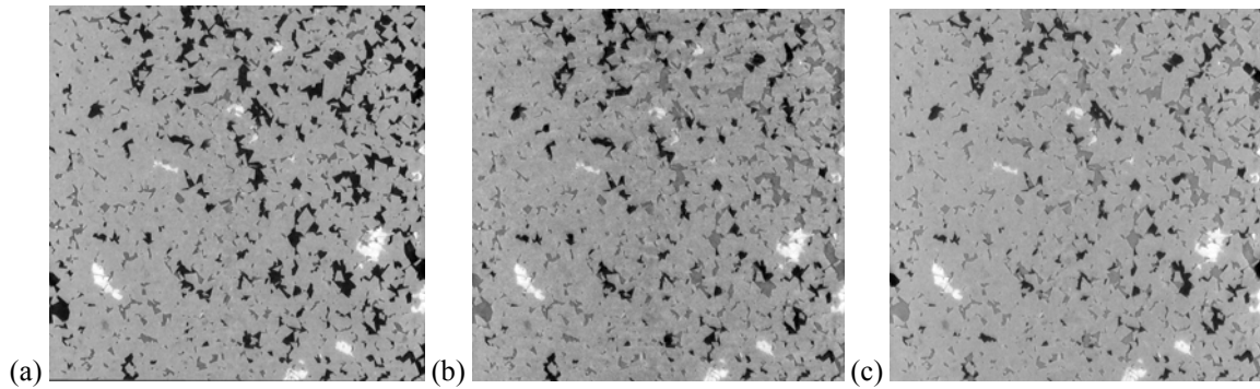
Figure 8: Slice of 3D \mu -CT image of sucrosic dolomite; (a) after drainage; (b) registered slice after SI; (c) after FI at Ca \sim 2 \times 10^{-4} ; oil phase is black and water phase is the grey intermediate between oil and the dolomite matrix.
