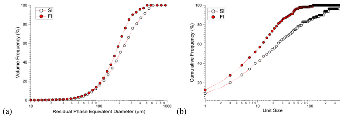
Figure 10: (a) Equivalent Diameter of the residual phase after SI and FI; Note that the larger clusters have been mobilized after FI while the smaller clusters remain. (b) Unit Size distribution.
