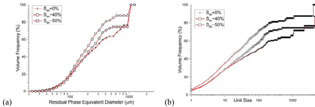
Figure 7: (a) Equivalent Diameter of the residual phase after drainage and SI on the bimodal carbonate sample; (b) Unit Size distribution. The larger trapped clusters at S_{wi} \sim 50\% compared to \sim 40\% may be due to the presence of thicker films at the higher S_{wi} leading to enhanced snap-off.
