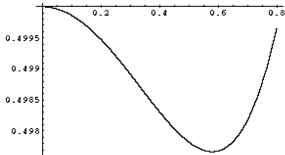
Fig. 13 Plot of the function \arcsin(\sqrt{(\sin x - x)^2 + (1 - \cos x)^2})/x^2 , verifying the last step of the proof of Lemma 4
