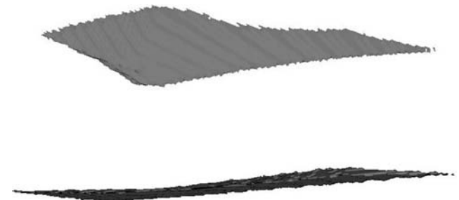
Fig. 5 For synthetic data with n = 20 points, the 3D shape of the remaining rotation region is shown after running the algorithm to resolution of 0.001 radians. Recall that the shape of the set of all rotations in the angle-axis representation is a closed 3-dimensional ball. The example in the figure is for a sideways motion of the camera with a field of view of about 60^\circ , and a motion equal to 0.5 times the distance to the closest point. The shape of the rotation region is quite flat and elongated. This is explained by the known translation/rotation ambiguity, that translation and rotation of a camera are at times difficult to distinguish, particularly for small fields of view
