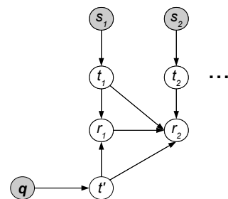
Figure 1: Graphical model used in PLMMR.
