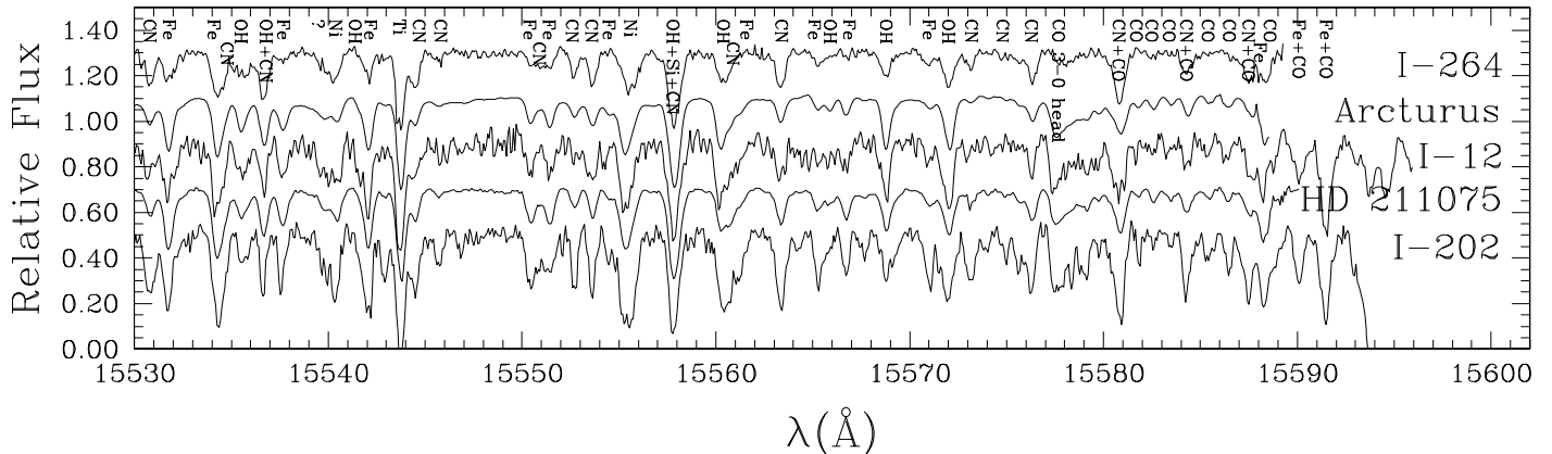
Fig. 1. Observed Phoenix spectra of selected bulge giants as well as thick (Arcturus = HD 124897) and thin (HD 211075) disk stars.
