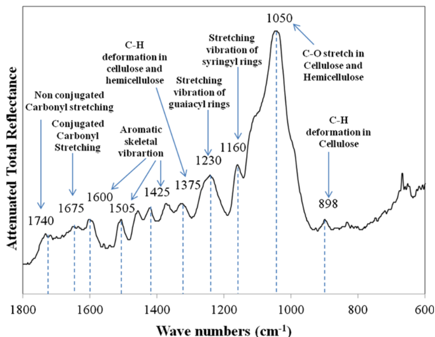
Figure 3. FT-IR spectra of untreated bamboo ( P. pubescens ).
