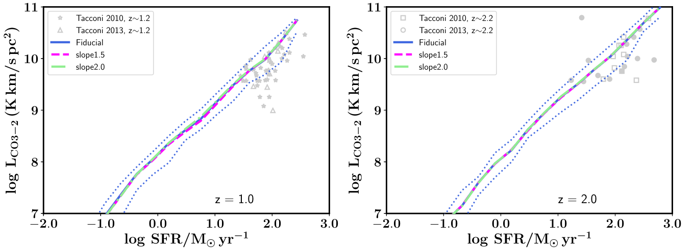
Figure C3. The CO J=3–2 luminosity of galaxies at z=1 and 2 as a function of their SFR for a model variant with a slope \beta of the cloud mass distribution function of \beta = 1.8 (Fiducial), \beta = 1.5 (slope1.5), and \beta = 2.0 (slope2.0). This figure is similar to Fig. 8. Different choices for the slope of the molecular cloud mass distribution function do not affect the predicted CO luminosity of galaxies.
