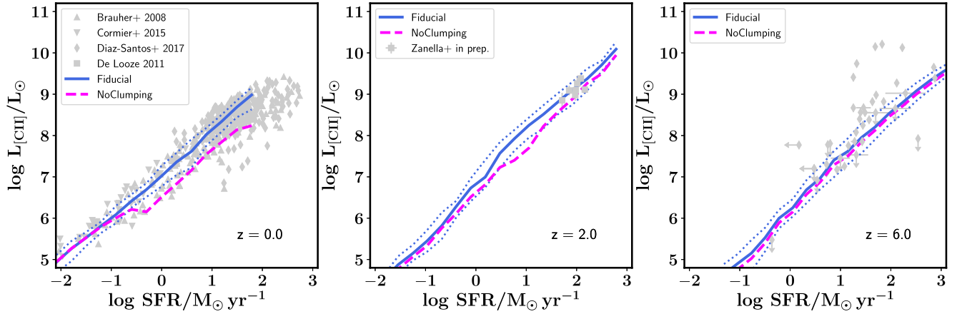
Figure B1. The [C II] luminosity of galaxies as a function of their SFR at z = 0, 2, and 6 for a model variant with (Fiducial) and without (NoClumping) turbulence dependent clumping. This figure is similar to Fig. 6. Clumping has a minimal effect on the predicted [C II] luminosities of galaxies.
