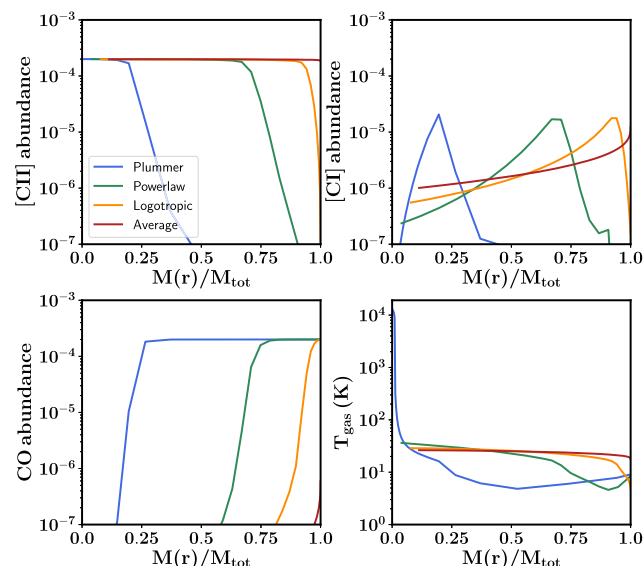
Figure 3. The [C II] (top left), [C I] (top right), and CO (bottom left) abundance and gas temperature (bottom right) profiles of a molecular cloud for different molecular cloud density profiles. The molecular cloud has a fixed mass of 10^5 M_{\odot} , an external pressure acting upon it of P_{\text{ext}}/k_B = 10^4 \text{ cm}^{-3} \text{ K} , a UV radiation field shining on it of one G_0 , and a solar metallicity. The different density profiles lead to very different radial profiles for the CO, [C I], and [C II] abundance and temperature of the gas.
