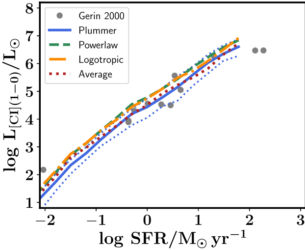
Figure 13. The [C I] 1–0 luminosity of galaxies at z = 0 as a function of their SFR assuming different radial density profiles for the gas within molecular clouds a fixed external pressure acting on the molecular clouds of P_{\text{ext}}/k_B = 10^4 \text{ cm}^{-3} \text{ K} . This figure is similar to Fig. 9. When imposing a constant external pressure on the cloud the [C I] luminosities predicted by the various density profiles are almost identical.
