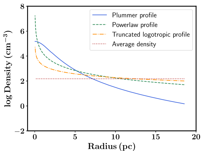
Figure 2. A representation of the four different density distribution functions within molecular clouds adopted in this paper. These were obtained assuming a molecular cloud with a mass of 10^5 M_{\odot} and an external pressure acting upon this molecular cloud of P_{\text{ext}}/k_B = 10^4 \text{ cm}^{-3} \text{ K} . One can clearly see the differences in minimum and maximum densities achieved in the inner and outer regions of the molecular cloud between the different profiles.
