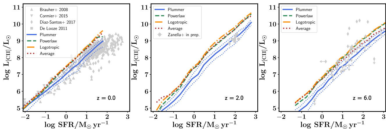
Figure 6. The [C II] luminosity of galaxies as a function of their SFR at z = 0, 2, and 6, assuming different radial density profiles for the gas within molecular clouds. Model predictions are compared to observational constraints (Brauer, Dale & Helou 2008; de Looze et al. 2011; Cormier et al. 2015; Díaz-Santos et al. 2017; Capak et al. 2015; Knudsen et al. 2016; Willott et al. 2015; Decarli et al. 2017; González-López et al. 2014; Kanekar et al. 2013; Pentericci et al. 2016; Bradač et al. 2017; Schaerer et al. 2015; Maiolino et al. 2015; Ota et al. 2014; Inoue et al. 2016; Knudsen et al. 2017; Carniani et al. 2017; Zanella et al. 2018). In this particular plot, the Plummer model represents our fiducial model. Changing the density profile of molecular clouds can lead to variations up to \sim 0.5 dex in the predicted [C II] luminosity of actively star-forming galaxies.
