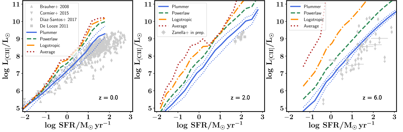
Figure 10. The [C II] luminosity of galaxies as a function of their SFR at z = 0, 2, and 6 for different radial density profiles for the gas within molecular clouds and assuming a fixed external pressure acting on the molecular clouds of P_{\text{ext}}/k_B = 10^4 \text{ cm}^{-3} \text{ K} . This figure is similar to Fig. 6, aside from the fact that here we impose a constant external pressure on the cloud the predicted [C II] luminosities increase.
