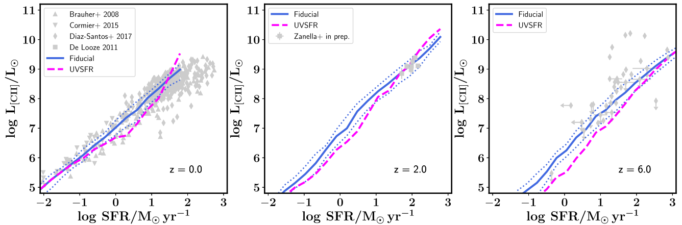
Figure 14. The [C II] luminosity of galaxies as a function of their SFR at z = 0, 2, and 6 for a model variant where the UV radiation field and CR strength are scaled as a function of the local SFR surface density (Fiducial) and as a function of the global galaxy SFR (UVSFR). This figure is similar to Fig. 6 aside from the varying relationship between the UV field and the SFR imposed in this figure. It is clear that a relationship that ties the UV field to the global SFR of galaxies underpredicts the [C II] luminosity at z = 0 for galaxies with an SFR less than 40 M_{\odot} \text{ yr}^{-1} and at high-redshift z = 6 . It furthermore predicts [C II] luminosities for z = 0 galaxies with SFRs higher than 40 M_{\odot} \text{ yr}^{-1} that are too bright. Tying the UV flux to \Sigma_{\text{SFR}} results in predictions in good agreement with the observational constraints.
