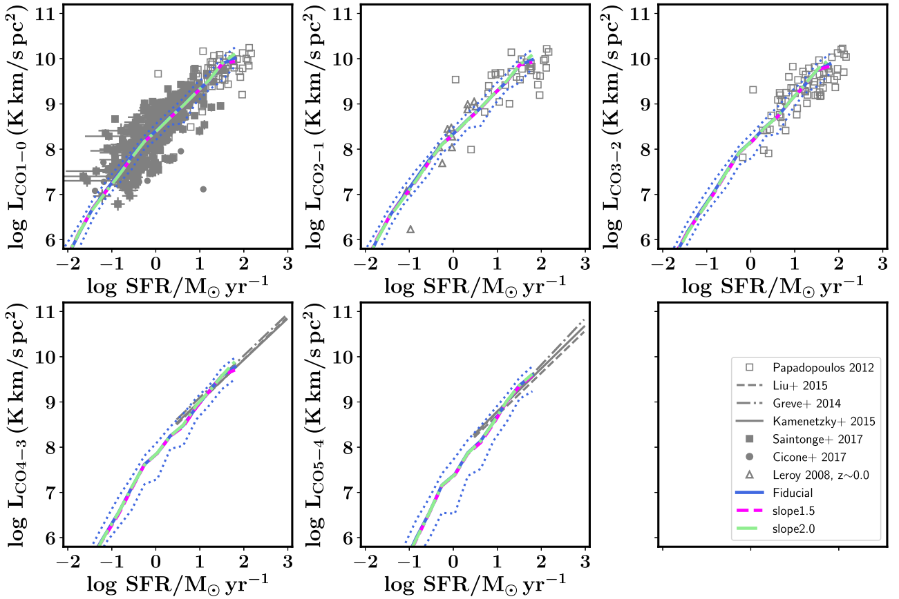
Figure C2. The CO J=1–0 to 5–4 luminosity of galaxies as a function of their SFR at z=0 for a model variant with a slope \beta of the cloud mass distribution function of \beta = 1.8 (Fiducial), \beta = 1.5 (slope1.5), and \beta = 2.0 (slope2.0). This figure is similar to Fig. 7. Different choices for the slope of the molecular cloud mass distribution function do not affect the predicted CO luminosity of galaxies.
